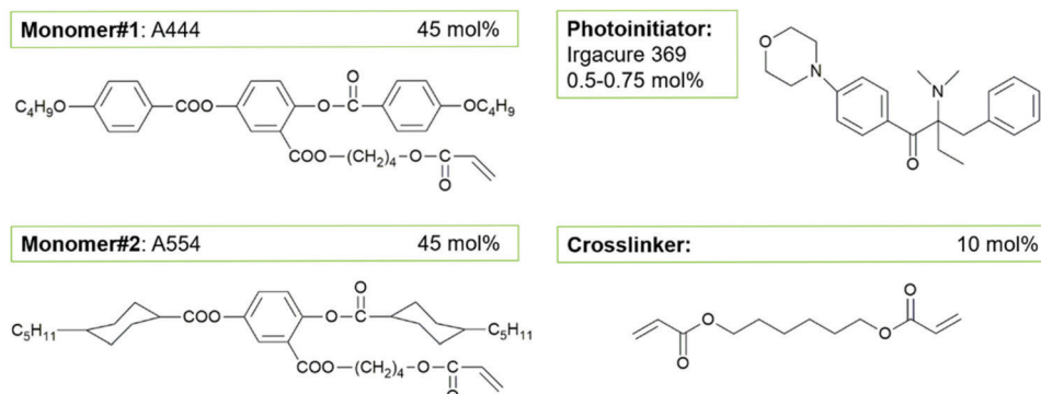
Fig. 1 Chemical structures of the compounds and their percentages in the mixture used in the experiment. Two monomers, 4'-acryloyloxybutyl 2,5-(4'-butyloxybenzoyloxy)benzoate (A444) and 4'-acryloyloxybutyl 2,5-di(4'-pentylcyclohexyloxy)benzoate (A554), of equal molar percentage are used, which allows for the formation of a mixture with a nematic phase at room temperature (25 °C). The rest of the mixture consists of the crosslinker 1,6-hexanediol diacrylate at 10 mol% and the trace amount of photoinitiator, 2-benzyl-2-(dimethylamino)-4'-morpholinobutyrophenone (Irgacure 369).
