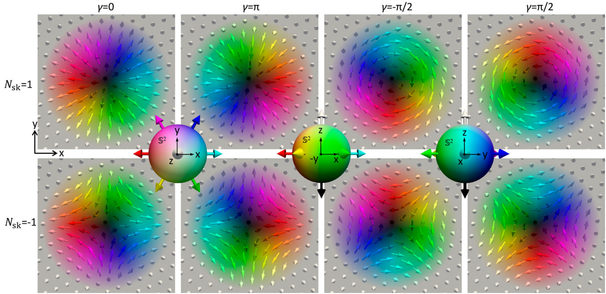
Figure 8. Full elementary skyrmions in magnetic systems. 2D Magnetic skyrmions characterized by the skyrmion number N_{sk} and helicity \gamma . All arrows are colored according to their orientations in the order parameter space \mathbb{S}^2 shown in the insets.
