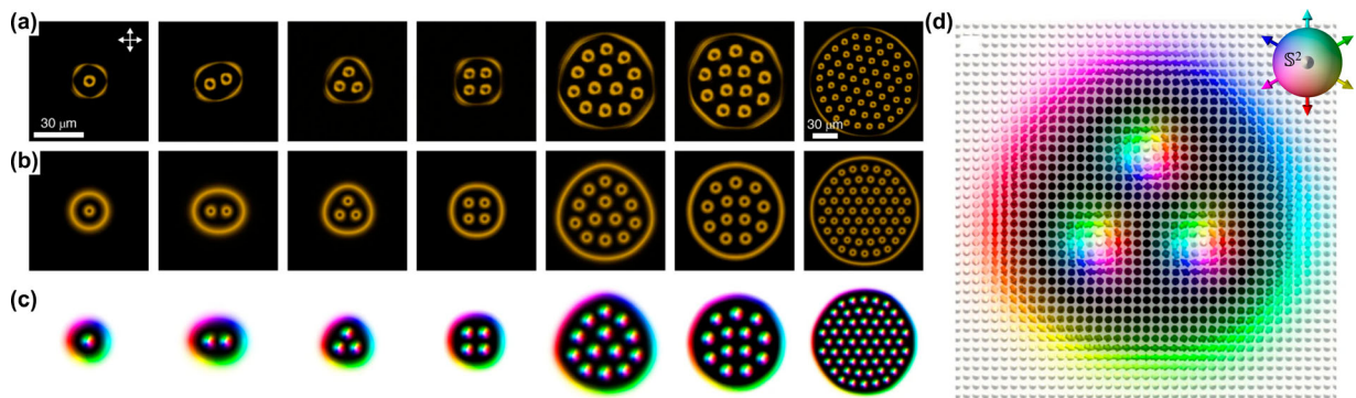
Figure 13. 2D skyrmions and skyrmion bags. (a) Polarizing optical micrographs of skyrmion bags with antiskyrmions inside, two stable conformations of the bag with 13 antiskyrmions inside (images 5 and 6 from the left), and the bag with 59 antiskyrmions within it (right-side image). (b,c) Computer-simulated counterparts of the skyrmion bags in (a). Crossed polarizers for (a,b) are marked by white double arrows in (a). (d) Close-up view of a computer-simulated bag with three antiskyrmions shown by colored, vectorized alignment field. Reproduced with permission from Ref. [123].
