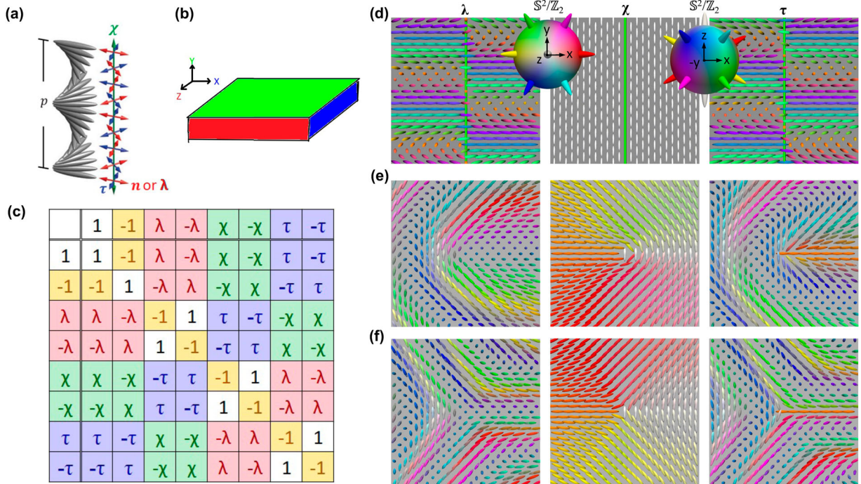
Figure 6. The topology of disclinations in CLCs. (a,b) The symmetry of the building blocks in cholesterics (a) and biaxial nematics (b) illustrated by the orthonormal frames \lambda, \chi, \tau and \mathbf{x}, \mathbf{y}, \mathbf{z} , respectively. (c) The multiplication table of the quaternion group Q_8 . All topologically stable disclinations in CLCs are characterized by one of the eight group elements, or one of the five conjugacy classes distinguished by colors. (d–f) Numerical visualizations of the \lambda(\mathbf{r}) , \chi(\mathbf{r}) , and \tau(\mathbf{r}) director fields along a \chi disclination (d), perpendicular to a \lambda^{+1/2} line (e), or a \lambda^{-1/2} line (f). The long green tube in (d) marks the core of the \chi disclination. All directors are colored according to their orientations in the nonpolar order parameter space as shown in the insets in (d).
