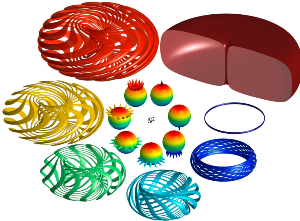
Figure 16. Tiling and linking of preimages of \mathbb{S}^2 points within a hopfion. Preimages of different azimuthal \mathbf{m} -orientations tile into tori for the same polar angles, with the smaller tori nesting inside bigger tori; the largest torus contains the north-pole preimage in its exterior corresponding to \mathbf{m}_0 and the other preimages nested within its interior. Reproduced with permission from Ref. [4].
