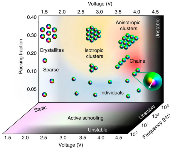
Figure 21. Schools of skyrmions characterized by a diagram of static and dynamic skyrmion assemblies and schools versus packing fraction, frequency f_c and voltage U . The configurations shown in the insets are consistent across all f_c at which skyrmions are stable. Reproduced with permission from Ref. [182].
