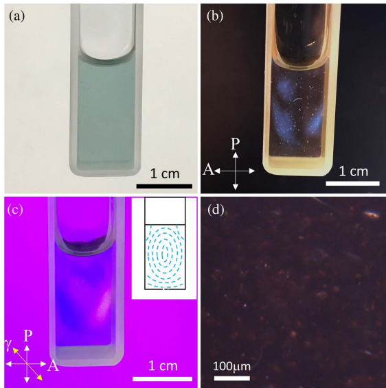
Fig. 2. (a) Optical photograph shows well-dispersed plasmonic DNA-origami in cellulose nanofiber solution without any aggregation or phase separation. (b) and (c) Weak optical birefringence of the plasmonic-LC composites is manifested under crossed polarizers (b) without and (c) with a 530 nm full waveplate, respectively. Inset in (c) schematically shows director field of the CNF-based LC. (d) Dark-field microscopy image shows that the plasmonic origami are well dispersed on the individual nanostructure basis.
