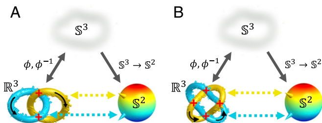
Fig. 1. Topological solitons. Preimages in \mathbb{R}^3 (and \mathbb{S}^3 ) correspond to distinct points on \mathbb{S}^2 form Hopf ( 2_1^2 ) (A) and Solomon links ( 4_1^2 ) (B) with linking numbers matching their Q = 1 (A) and Q = 2 (B) Hopf indices. Since the direct ( \phi ) and inverse ( \phi^{-1} ) stereographic projections relate smooth configurations in \mathbb{S}^3 and \mathbb{R}^3 when embedded within the uniform \mathbf{n}_0 and \mathbf{M}_0 , these solitons are characterized by the \mathbb{S}^3 \rightarrow \mathbb{S}^2 maps, the third homotopy group \pi_3(\mathbb{S}^2) = \mathbb{Z} and Q \in \mathbb{Z} . Black arrows indicate circulation directions, crossing signs are marked in red color, and the colors of preimages match that of the corresponding points on \mathbb{S}^2 .
