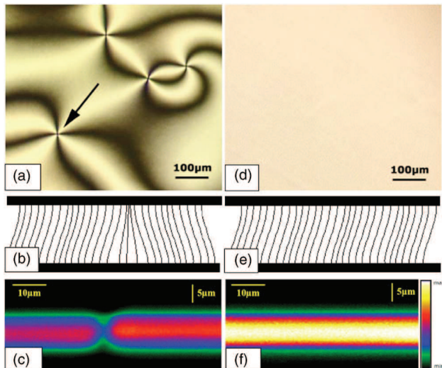
FIG. 1. Effect of rubbing of one plate on the director configurations in the VA cell: (a) Polarizing microscope texture, (b) director configuration of a VA cell with azimuthally degenerated homeotropic alignment at nonrubbed substrates, and (c) a FCPM image of the vertical cross section; (d)–(f) show the corresponding pictures for a rubbed VA cell. The cells are driven by pulses of 4.5 Vrms at 1 KHz. The arrow in (a) indicates an umbilic defect.
