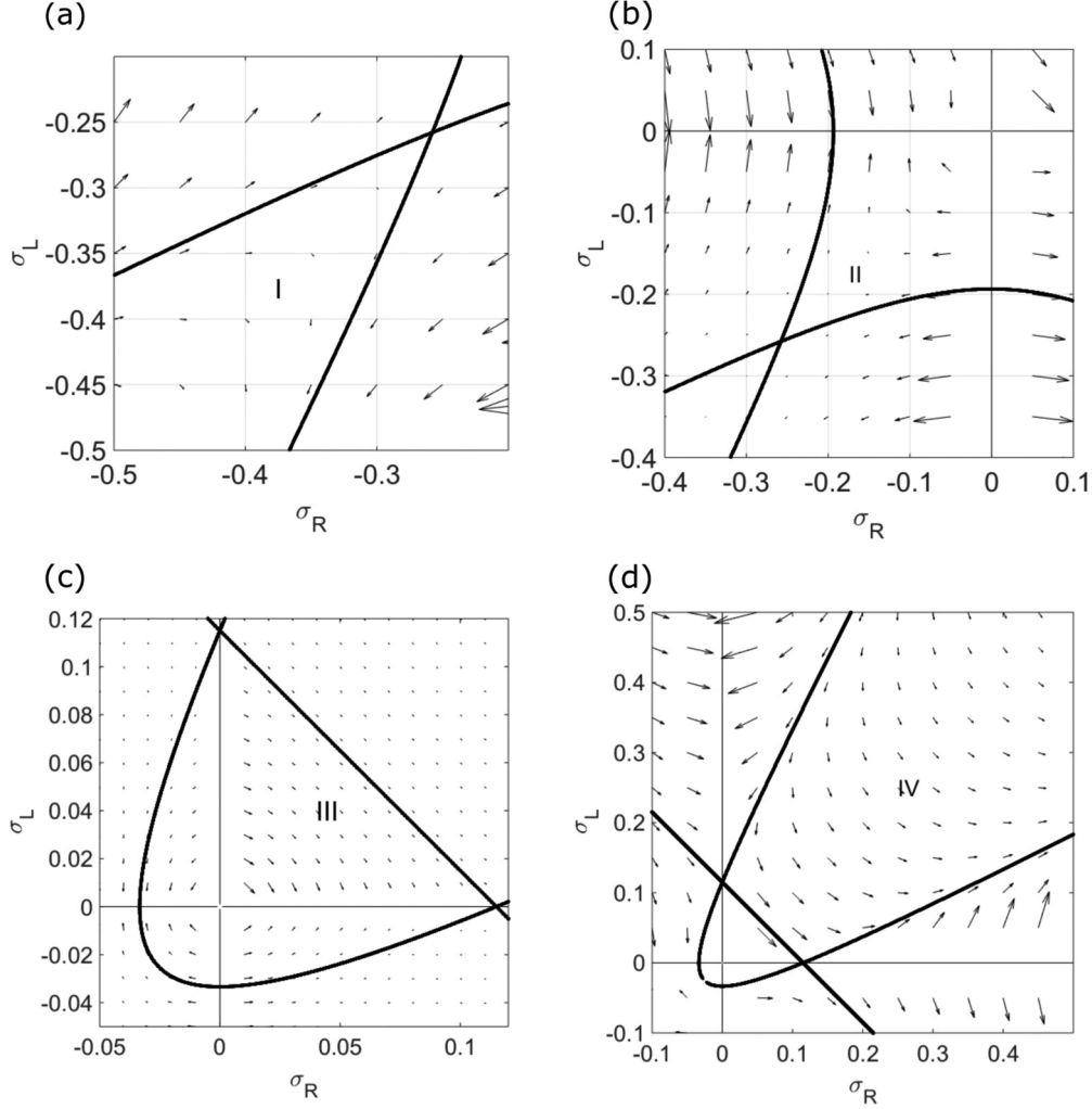
FIG. 5. Illustration of the four regions of the central density, as defined in the text. The switching rate is 0.5 \text{ s}^{-1} , the bulk motor concentration c = 200 \text{ nM} , and the motor speed is 5 \mu\text{m s}^{-1} ; other parameters are the reference values of Table I. Arrows indicate the vector field, which has the mathematical form of Eqs. (12) and (13).
