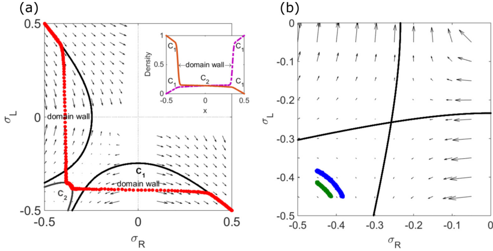
FIG. 4. Effects of domain walls and finite size on density profiles. Left, determination of domain wall positions in the phase-plane trajectory and the density profile (inset). Red points show kMC simulation results. The boundary points are (\sigma_R, \sigma_L) = (-\frac{1}{2}, \frac{1}{2}) and (\sigma_R, \sigma_L) = (\frac{1}{2}, -\frac{1}{2}) . The solution locally follows the flow, which cannot connect the boundary points without crossing the lines with \sigma_R = 0 and \sigma_L = 0 where the velocity is ill defined. Crossing these lines uses the matching condition to connect to another exact solution curve, introducing a domain wall. Inset shows the density profiles of \rho_R (purple, dashed) and \rho_L (brown, solid). The sharp transitions in \rho_R and \rho_L indicate the domain walls. There are three regions which are separated by two domain walls: regions near ends follow C_1 , and the region at the center is described by C_2 . Right, finite-size constraint. The blue points (longer curve) are kMC simulation results for N = 1000 , and the green (shorter curve) N = 500 . For a larger number of sites, the dimensionless motor speed is smaller, moving the solution closer to the LI. The switching rate is 0.44 \text{ s}^{-1} (left), 0.1 \text{ s}^{-1} (right), the bulk motor concentration c = 200 \text{ nM} , and the motor speed 5 \mu\text{m s}^{-1} ; other parameters are the reference values of Table I. Arrows indicate the vector field, which has the mathematical form of Eqs. (12) and (13).
