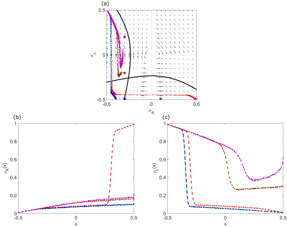
FIG. 18. Example phase-plane trajectories and density profiles for general boundary conditions, illustrating how altering the right boundary condition changes the density profile. (a) Colored dots indicate the right boundary condition. Red curve satisfies all four boundary conditions; green, blue, and brown curves do not satisfy \beta_R ; and the purple curve satisfies \alpha_R and \beta_L . (b), (c) Corresponding density profiles on the R lane (b) and L lane (c). The switching rate is 0.1 \text{ s}^{-1} , bulk motor concentration c = 200 \text{ nM} , and motor speed 5 \mu\text{m s}^{-1} ; other parameters are the reference values of Table I. Arrows in (a) indicate vector field, which has the mathematical form in (12) and (13).
