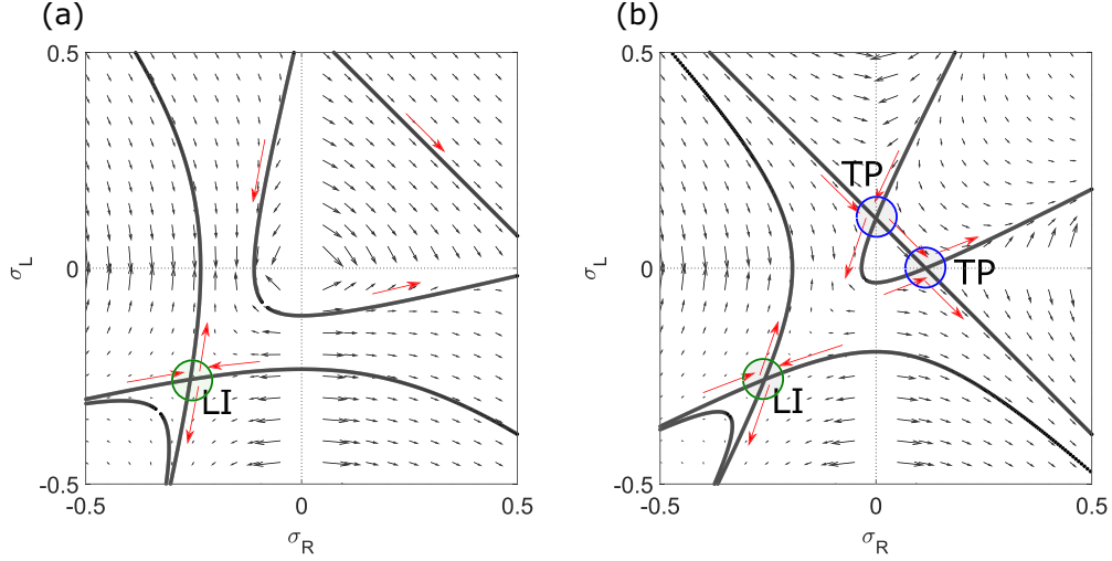
FIG. 2. Flows in the \sigma_R - \sigma_L phase plane for low [(a), 0.1 \text{ s}^{-1} ] and high [(b), 0.5 \text{ s}^{-1} ] switching rates. Solid lines are trajectories that pass through the fixed points, as discussed in the text. The Langmuir isotherm is labeled LI and the transition points TP. The bulk motor concentration is 200 nM, the motor speed is 5 \mu\text{m s}^{-1} , and other parameters are the reference values of Table I. Arrows indicate the vector field, which has the mathematical form of Eqs. (12) and (13).
