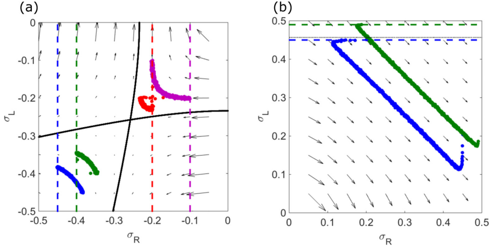
FIG. 8. Example phase-plane trajectories of L and H phases. (a) L phase. The starting and ending points are (\sigma_R, \sigma_L) = (-0.45, -0.4) and (-0.4, -0.45) (blue), (-0.4, -0.45) and (-0.45, -0.4) (green), (-0.2, -0.1) and (-0.1, -0.2) (red), and (-0.1, -0.2) and (-0.2, -0.1) (purple). The dashed lines show that the L phase obeys the left boundary conditions, where the positions are \sigma_R = -0.45 (blue), \sigma_R = -0.4 (green), \sigma_R = -0.2 (red), and \sigma_R = -0.1 (purple). (b) H phase. The starting and ending points are (\sigma_R, \sigma_L) = (0.3, 0.45) and (0.45, 0.3) (blue), (0.2, 0.49) and (0.49, 0.2) (green). The dashed lines show that the H phase obeys the right boundary conditions, where the positions are \sigma_L = 0.45 (blue) and \sigma_L = 0.49 (green). The black dashed line \sigma_L = \rho_c - \frac{1}{2} \approx 0.4567 , the critical density \rho_c (see text) of the local minimum and local maximum phases. The switching rate is 0.1 \text{ s}^{-1} , bulk motor concentration c = 200 \text{ nM} , and motor speed 5 \mu\text{m s}^{-1} ; other parameters are the reference values of Table I. Arrows indicate the vector field, which has the mathematical form of Eqs. (12) and (13).
