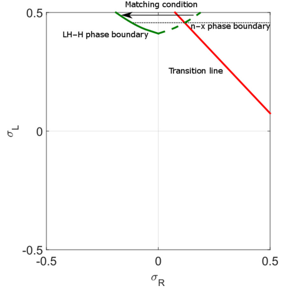
FIG. 14. Illustration of calculation of phase boundaries of local maximum and minimum phases. The dashed green line is obtained from backward integration of the \sigma_R = \sigma_L line to x = -\frac{1}{2} . The green line indicates the LH phase boundary determined by the matching condition, where the right of the line is the H phase. The red line is the transition line. Since the H phase satisfies the right boundary condition, the starting point of the density profile depends on \sigma_L value. Therefore, the phase boundary of the local maximum and minimum phase is a horizontal line that intersects the green dashed line and the transition line. The local minimum phase is above the black dashed line. The switching rate is 0.1 \text{ s}^{-1} , bulk motor concentration c = 200 \text{ nM} , and motor speed is 5 \mu\text{m s}^{-1} ; other parameters are the reference values of Table I.
