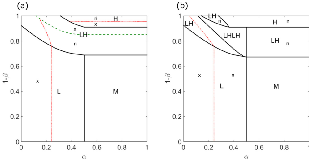
FIG. 9. The phase diagrams for low [(a), 0.1 \text{ s}^{-1} ] and high [(b), 0.5 \text{ s}^{-1} ] switching rates. The phases are L (low density), M (Meissner), H (high density), LH (low-density-high-density coexistence), and LHLH (low-density-high-density-low-density-high-density coexistence). The thick green dashed line indicates where the domain wall position x_w = 0 , which separates regions with a local maximum of the central density ( x ) or local minimum ( n ). The red dashed lines indicate boundaries between local maximum and minimum phases. For low switching rate, the left parts of the L and LH phases are local maximum phases, and the right are local minimum phases. The upper part in the H phase is local minimum phase. For high switching rate, the left parts of the L and LH phases are local maximum phases, and the right parts are local minimum phases. The bulk motor concentration is c = 200 \text{ nM} , and the motor speed 5 \mu\text{m s}^{-1} ; other parameters are the reference values of Table I.
