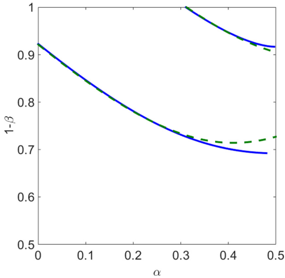
FIG. 16. Comparison of determination of the L phase boundaries using the total binding constraint with linear approximation [green dashed curves, Eqs. (27) and (31)] and the finite-size constraint without any approximation (blue solid curves). The switching rate is 0.1 \text{ s}^{-1} , bulk motor concentration c = 200 \text{ nM} , and motor speed 5 \mu\text{m s}^{-1} ; other parameters are the reference values of Table I.
