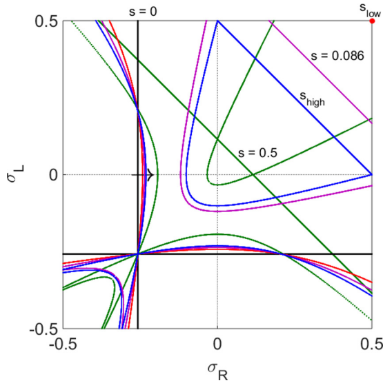
FIG. 3. Changes in trajectories and fixed points with varying switching rate. Curves with s = 0 \text{ s}^{-1} , black; s = \frac{3(k_{\text{off}} - k_{\text{on}})}{4} \approx 0.0862 \text{ s}^{-1} , purple; s = s_{\text{high}} \approx 0.1150 \text{ s}^{-1} , blue; s = 0.5 \text{ s}^{-1} , green. The red point labels s_{\text{low}} . The arrow indicates how the curve with C_{LI} changes as s increases. The bulk motor concentration is c = 200 \text{ nM} and motor speed is 5 \mu\text{m s}^{-1} ; other parameters are the reference values of Table I.
