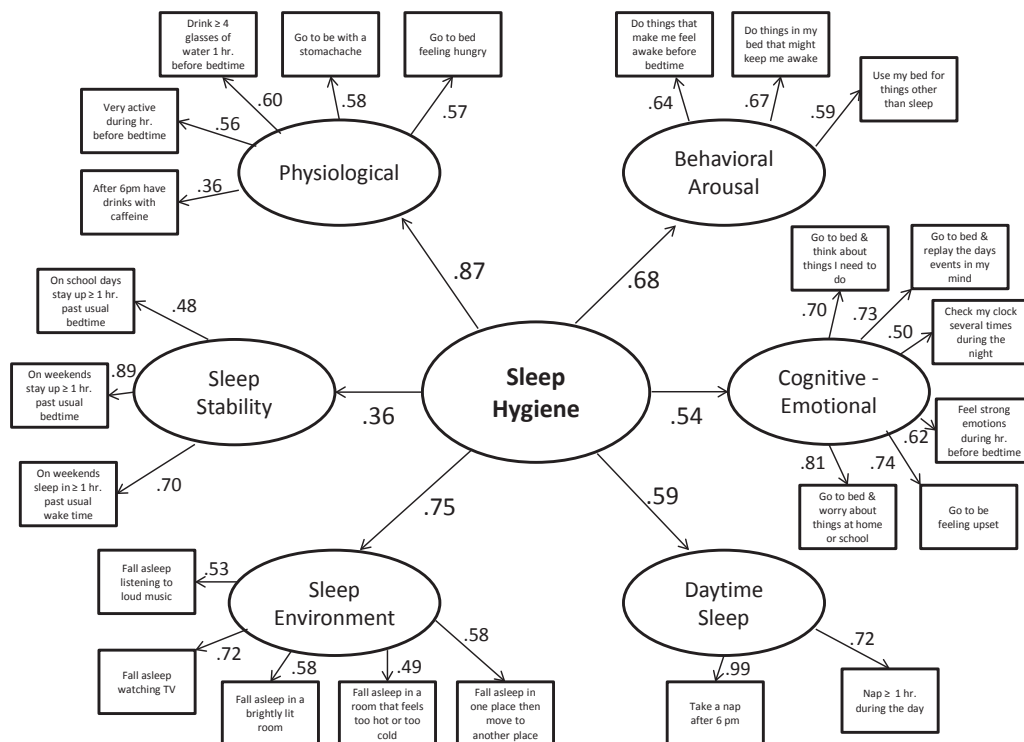
Figure 1. Factor structure of the revised 24-item Adolescent Sleep Hygiene Scale and factor loadings from the second-order factor analysis.
