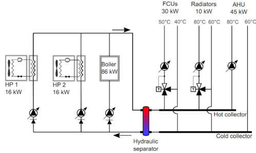
Fig. 1 heating system with heat production on the left hand side and heat emission on the right hand side coupled by a pressure balancing tank.
