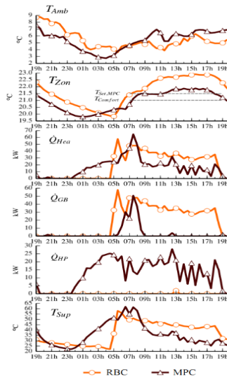
Fig. 3 Comparison of RBC and MPC quantities (from top to bottom): the ambient temperature around the building ( T_{Amb} ), the average zone temperature in the building ( T_{Zon} ), the total heat going to the zones ( Q_{Hca} ), heat production gas boiler ( Q_{GB} ), heat production heat pumps ( Q_{HP} ), supply water temperature ( T_{Sup} ).
