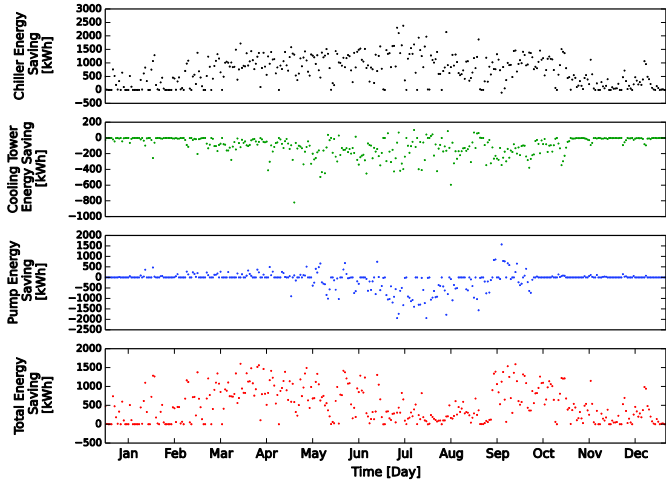
Fig. 5 Daily energy saving by the MPC compared to the conventional chiller stage control
