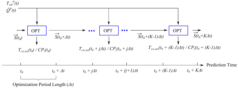
Fig. 4 the MPC framework for chillers
