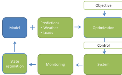
Fig. 2 the MPC framework for heat pumps
