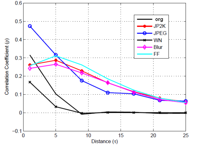
Fig. 10. Plot of spatial correlation coefficient ( \rho(\tau) ) for various distance \tau for one subband of an image, across distortions.
