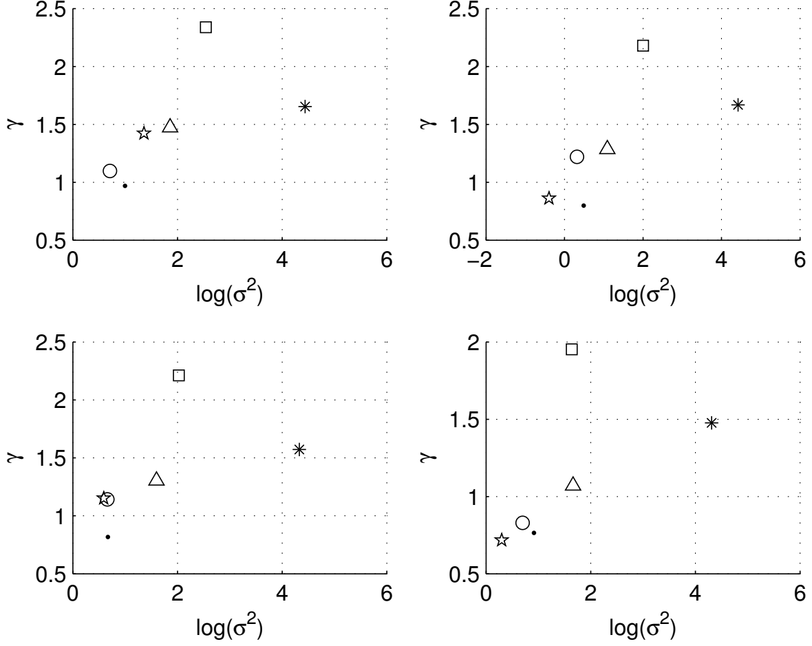
Fig. 6. Plot of \log_e(\sigma^2) vs. \gamma for d_1^{120^\circ} for each of the images considered in Fig. 2 and their associated distorted versions. Notice how each distortion seems to cluster in a particular region, immaterial of the image content. Images (a)-(d): left to right, top to bottom. Reference image ( \square ), JPEG ( \circ ), JPEG2K ( \Delta ), WN ( * ), blur ( \cdot ) and ff ( \star ).
