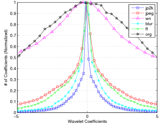
Fig. 5. Subband statistics from d_1^{0^\circ} of the image in Fig. 2 (c) for different distortions. Notice how each distortion affects the statistics in a characteristic way.
