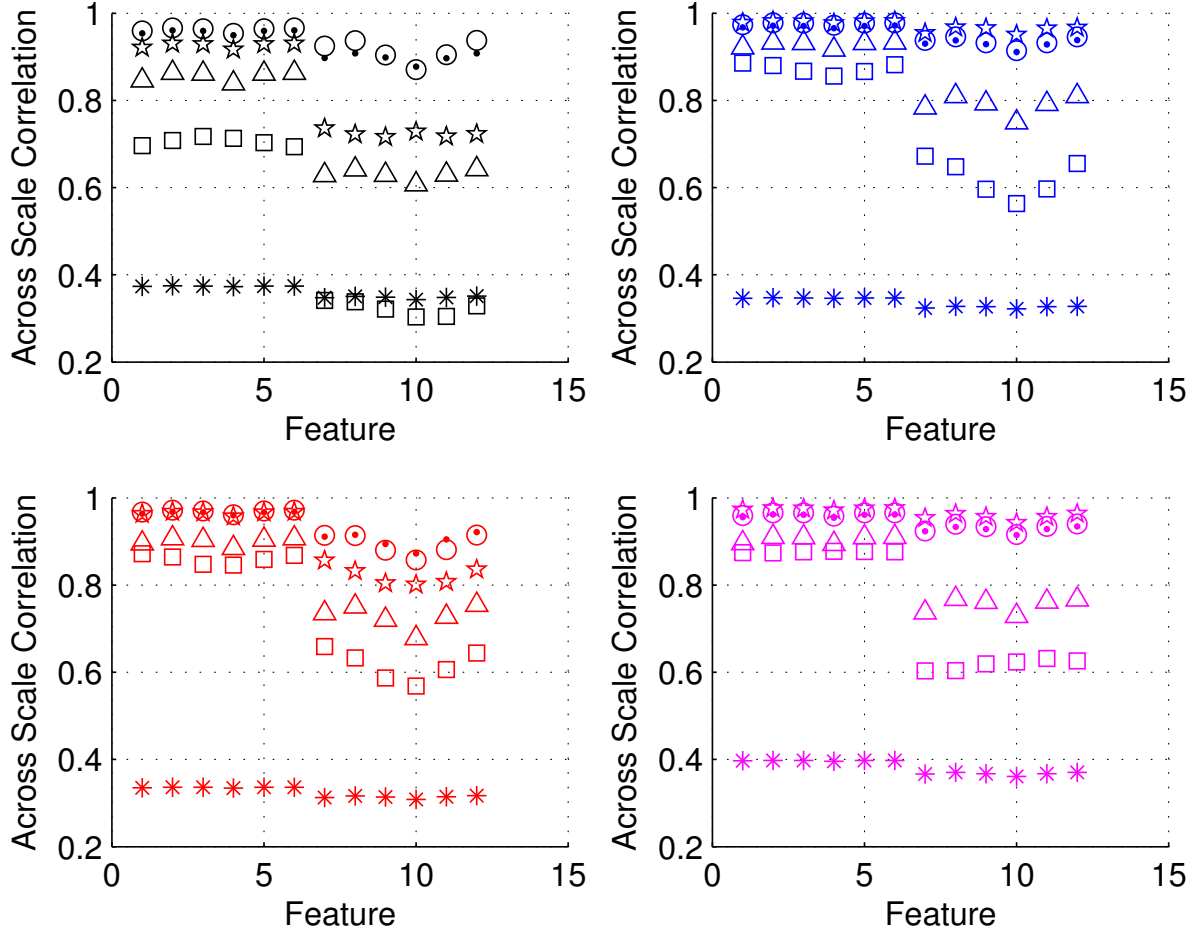
Fig. 9. Across scale correlation statistics for reference and distorted images. Images (a)-(d): left to right, top to bottom. Reference image ( \square ), JPEG ( \circ ), JPEG2K ( \Delta ), WN ( * ), blur ( \cdot ) and ff ( \star ). 1 – 12 on the x -axis correspond to f_{32} - f_{43} .
