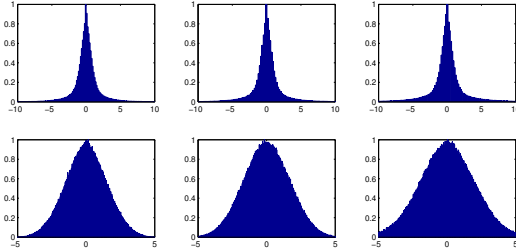
Fig. 4. Figure demonstrating the effect of divisive normalization on the subband statistics of image in Fig. 2(a). The first row shows the histogram of subband coefficient distributions before divisive normalization, while the second row is the distribution after normalization. Divisive normalization makes the subband statistics of natural images more Gaussian-like, as compared to the Laplacian nature of the pre-normalized subband coefficients.
