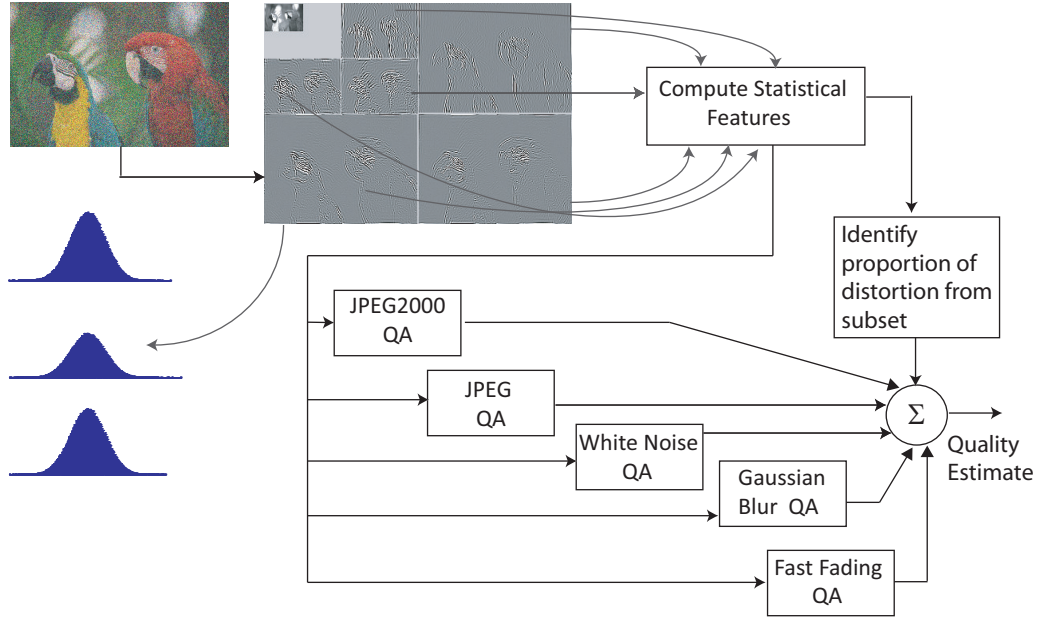
Fig. 1. The proposed Distortion identification-based Image Verity and Integrity Evaluation (DIIVINE) index consists of two stages: probabilistic distortion identification followed by distortion-specific quality assessment as illustrated here.
