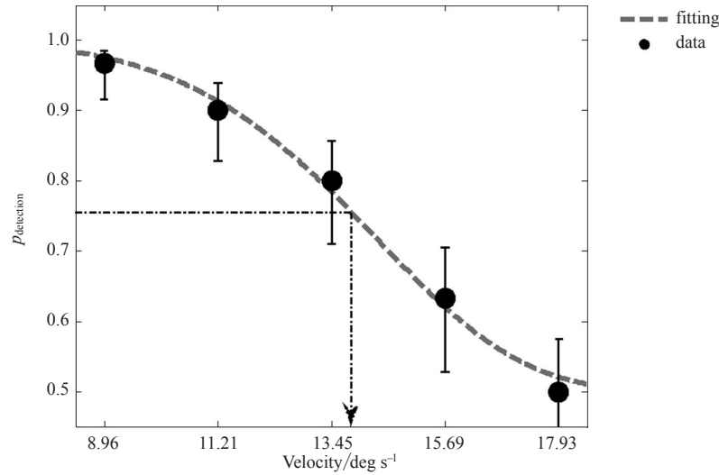
Figure 2. Psychometric data fitted to the Weibull function. The x-axis is rotational velocity (in deg s -1 ), and the y-axis is a probability of detection ( p_{\text{detection}} ). The velocity corresponding to a probability of detection equal to 0.75 was chosen as the threshold of velocity for silencing, v_{\text{th}} . Error bars using the binomial distribution with 68% confidence intervals are shown.
