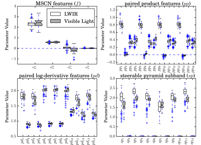
Fig. 8. Box plot comparison of features between natural LWIR and natural visible light images. The notches indicate 95 percent confidence intervals about the median.
