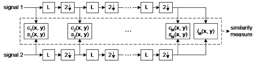
Fig. 1. Multi-scale SSIM. L = low-pass filtering, 2 \downarrow = downsampling by 2.
