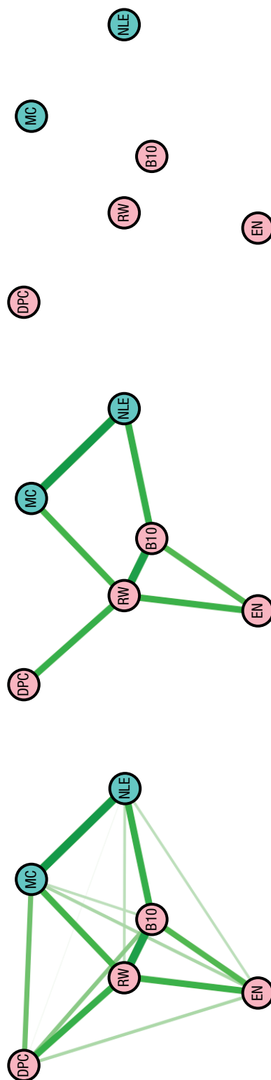
Fig. 4. Estimated network structures of the six place-value tasks across varying levels of edge-weight thresholds, separately for kindergarten knowledge and first-grade knowledge. The six nodes (i.e., place-value tasks) are represented by circles, and the edges are represented as lines. All edge weights are positive. Thicker lines indicate stronger edge weights or partial-correlation coefficients. A threshold of 0 indicates no threshold, so all estimated pathways are displayed. A threshold of .2 allows estimated edge weights that are above .2 to be shown, whereas a threshold of .4 allows edge weights above a .4 threshold to be shown. Multidimensional scaling was used to visualize the network edges estimated from the graphical “least absolute shrinkage and selection operator” (LASSO) network but with spacing based on zero-order correlations. Consequently, nodes that are close together are similar in terms of zero-order correlations, but nodes that share thick edges are similar in terms of regularized partial correlations. The border color of the node represents the predicted network cluster (i.e., a dark red border illustrates predicted count + unit syntax tasks; a dark turquoise border illustrates predicted approximate tasks). The fill color of the node represents the resulting estimated network clusters from the cluster analysis (i.e., the pink fill illustrates resulting count + unit tasks; the turquoise fill illustrates resulting approximate tasks). For the first-grade knowledge network, the border color of all nodes is black because we expected the nodes to be more integrated and not form clusters; however, the cluster analysis yielded two clusters as illustrated by the fill colors. B10 = base-10 counting; EN = expanded notation; DPC = digit-place correspondence; NLE = number-line estimation; RW = reading/writing; MC = magnitude comparison.
