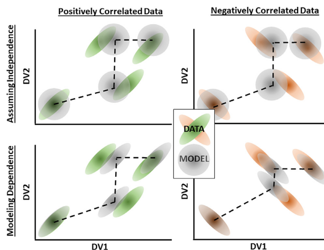
Fig. 1. Monotonicity assessment errors due to unacknowledged dependencies. Panels depict hypothetical datasets with differing patterns of correlation on two tasks (DV1, DV2), across four experimental conditions. Data from the experimental conditions are depicted with colored ellipses (green for a positive correlation and red for a negative correlation). The gray ellipses represent a hypothetical model of these data and are connected by an approximately best-fitting monotonic function in each case (dashed line). These functions were chosen by hand for illustrative purposes. The top row is a model that assumes independence between the two tasks whereas the bottom row is a model that estimates the correlation in the data. In these hypothetical examples, the standard deviations are assumed to be constant and known (all ellipses have equal standard deviation). Note that average performance per condition and variance for each task is identical in all situations. However, a model that only considers condition means and variances, but not covariances, neglects valuable information that could constrain model fitting. For instance, the bottom row shows that the best-fitting monotonic function fails to capture the middle two conditions in the case of positively correlated data but not negatively correlated data. . (For interpretation of the references to color in this figure legend, the reader is referred to the web version of this article.)
