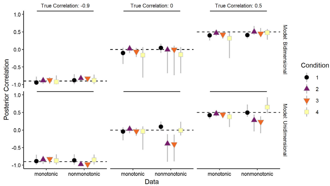
Fig. 5. Recovery of simulated trial-level correlation. Posterior distributions (median and 95% highest density interval) of each of the four trial-level correlation parameters (one for each condition) across the simulated datasets. The horizontal axis is grouped by whether the data were generated with a monotonic or non-monotonic function, and the top and bottom rows show the posteriors after fitting with the bidimensional and unidimensional models, respectively (the unidimensional model is nested within the bidimensional model). Most posterior distributions straddle the value that was used to generate the data (dashed line), but the largest misses occur when the data were not matched to the model.
