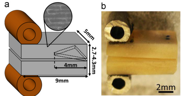
Fig. 2 – (a) Schematic of the chevron notch specimen with dimensions and (b) an actual image of a specimen made from top shell nacre.
