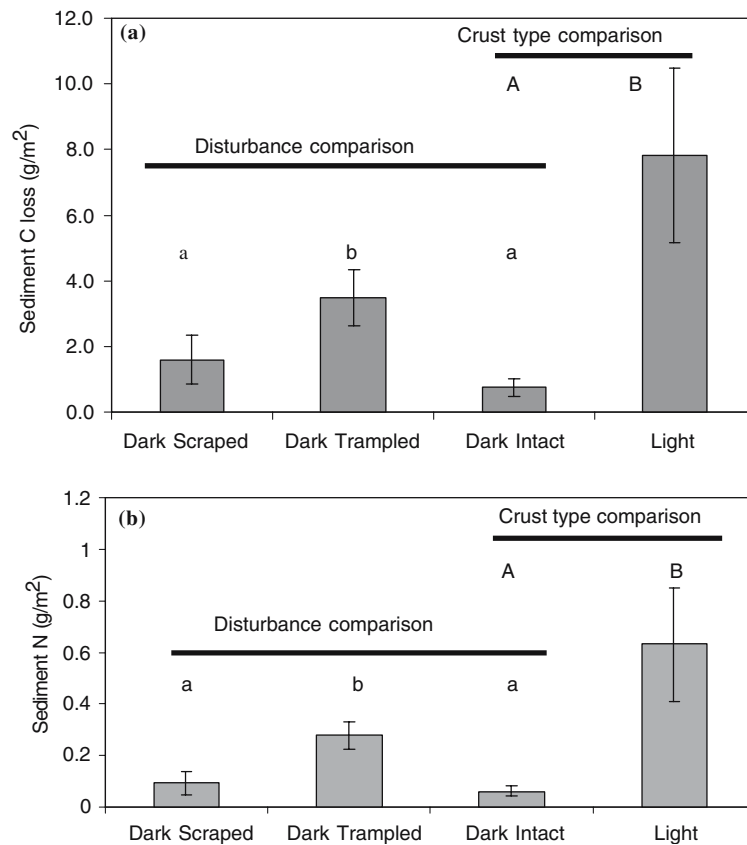
Figure 2. Sediment C and N losses. Above each bar, a lower case letter represents differences within the disturbance experiment, whereas capital letters signify treatment differences by crust type. If a different letter appears above a bar, means are significantly different at p < 0.10 .
