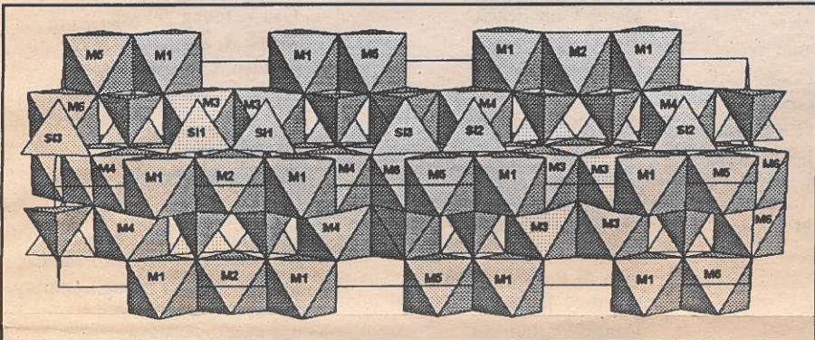
A [101] projection (b-horizontal) of the crystal structure of hydrous wadsleyite II. Octahedral sites are M1, M2, M3, M4, M5, and M6. Tetrahedral sites are Si1, Si2, and Si3.
