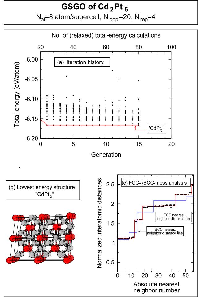
Figure 3. (a) GSGO of \text{Cd}_2\text{Pt}_6 ( N_{\text{pop}} = 20 , N_{\text{rep}} = 4 ). (b) The model of the ground-state structure found after 24 structure relaxations is \text{L1}_3 (space group No 65, Cmmm ): the underlying crystal lattice is fcc as evidenced by the fcc/bcc analysis shown in (c).
