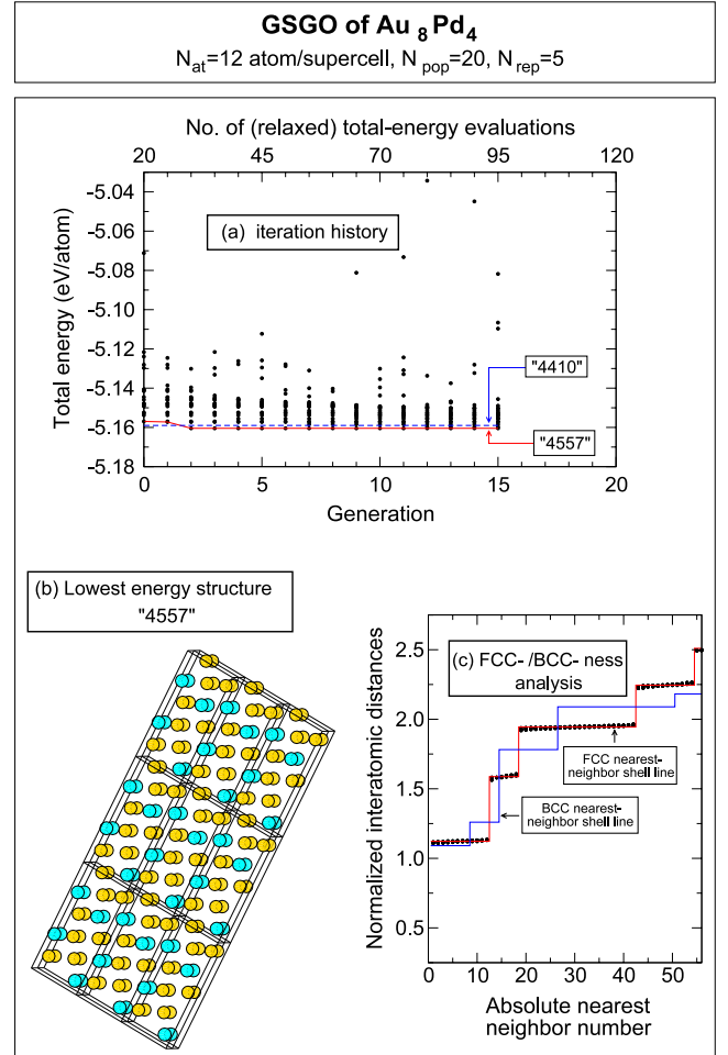
Figure 2. (a) History of the evolutionary optimization of \text{Au}_8\text{Pd}_4 ( N_{\text{pop}} = 20 and N_{\text{rep}} = 5 ). (b) The lowest-energy structure that was found after 30 structure evaluations (space group No 12, C2/m ). This structure has an fcc underlying lattice as shown by the fcc-/bcc-ness analysis of (c).
