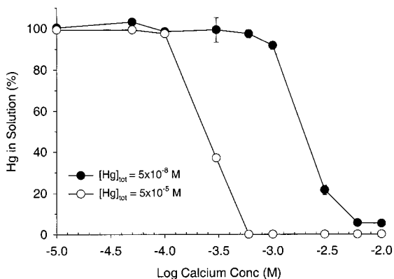
FIGURE 5. Effect of calcium concentration on the precipitation of metacinnabar at two different Hg concentrations (experiment 9): [\text{sulfide}]_{\text{total}} = 10^{-3} \text{ M} . Mercury concentration in solution is in the fraction that passes through a 0.1 \mu\text{m} filter.
