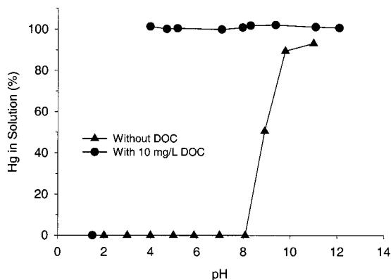
FIGURE 1. Effect of pH on the precipitation of metacinnabar (experiments 1 and 2 in Table 1): [\text{Hg}]_{\text{tot}} = 5 \times 10^{-5} \text{ M} ; [\text{sulfide}]_{\text{total}} = 10^{-3} \text{ M} . Mercury concentration in solution is in the fraction that passes through a 0.1 \mu\text{m} filter.
