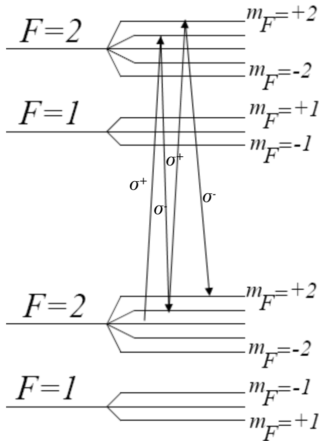
Figure A.6. Rubidium-87 hyperfine structure and magnetically sensitive sublevels. Typical transitions are shown for atoms undergoing optical pumping with \sigma^+ left-hand circularly polarized light under an applied magnetic field. While 5^2P_{1/2} to 5^2S_{1/2} decay transitions occur with \Delta m = 0, \pm 1 , because \sigma^+ light has angular momentum +\hbar , only \Delta m = +1 is allowed. This results in the atoms being pumped to the F=2 , m_F=+2 level.
