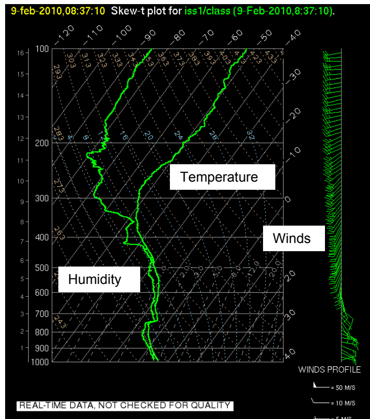
Figure 3.6. Radiosonde data at 08:37 UT at Fort Atkinson, WI. Altitude profile up to 16 km. Less inconsistency in winds at 500m altitude than wind profiler data.
