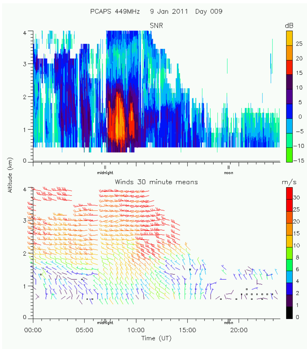
Figure 2.21. 449 MHz spaced antenna wind profiler data at West Jordan, Utah on 9 January 2011. SNR (dB) and horizontal winds (m/s).
