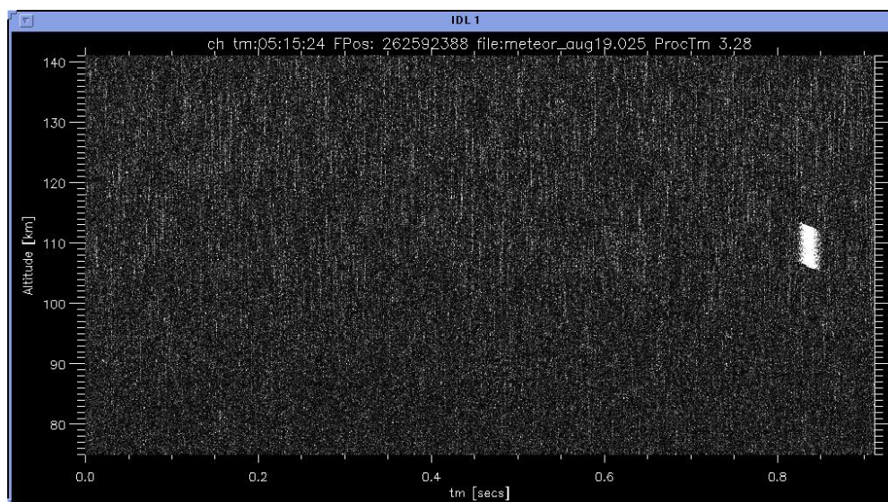
Figure 1.18. Plot of altitude vs. time showing a return from a single meteor at Arecibo Observatory.
