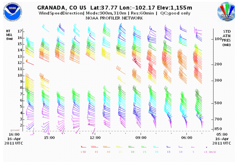
Figure 1.2. Example of wind profiler data from the Granada, Colorado station of the NOAA National Profiler Network.
