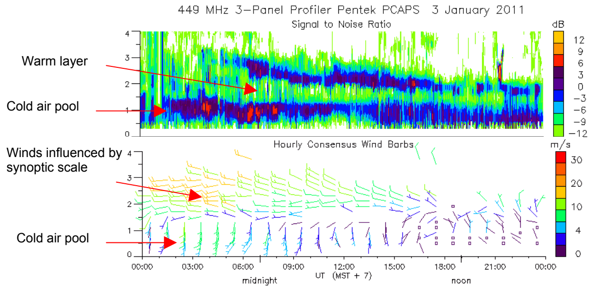
Figure 2.25. 449 MHz wind profiler data from Salt Lake City, Utah on 3 January 2011 showing persistent cold-air pool layers (top) and winds within the cold-air pool and winds influenced by the synoptic scale (bottom).
