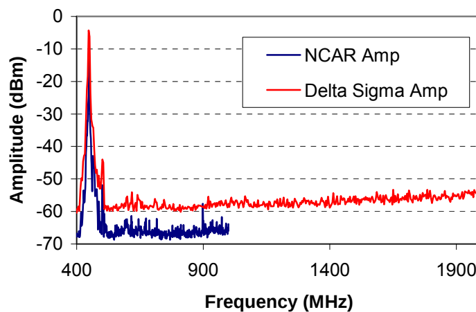
Figure 2.16. Measured radar output emissions vs. frequency using a patch antenna connected to a spectrum analyzer. Spectral output of 3 combined 1 kW modules is compared with a commercial 2 kW transmitter.
