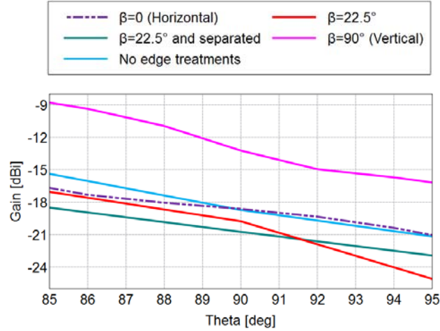
Figure 4.3. Simulation of E-plane sidelobe levels near the horizon between \theta=85 - 95^\circ using different configurations of clutter fence edge treatment. Note that \theta is the angle of the computed antenna pattern while \beta is the angle of the edge treatment.
