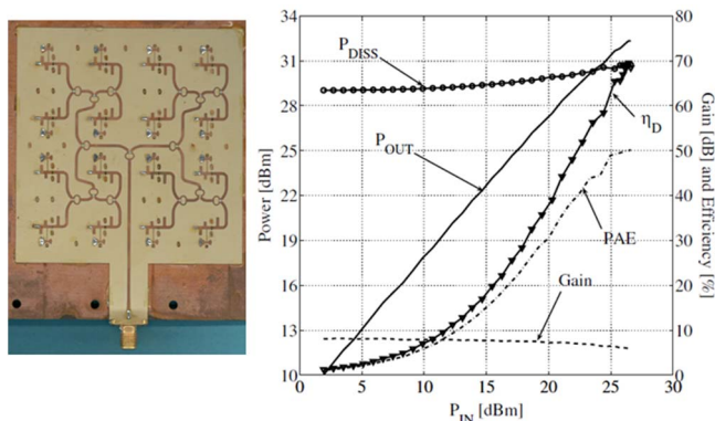
Fig.11. Spatial power combiner with class-E PAs at 10GHz [21].
