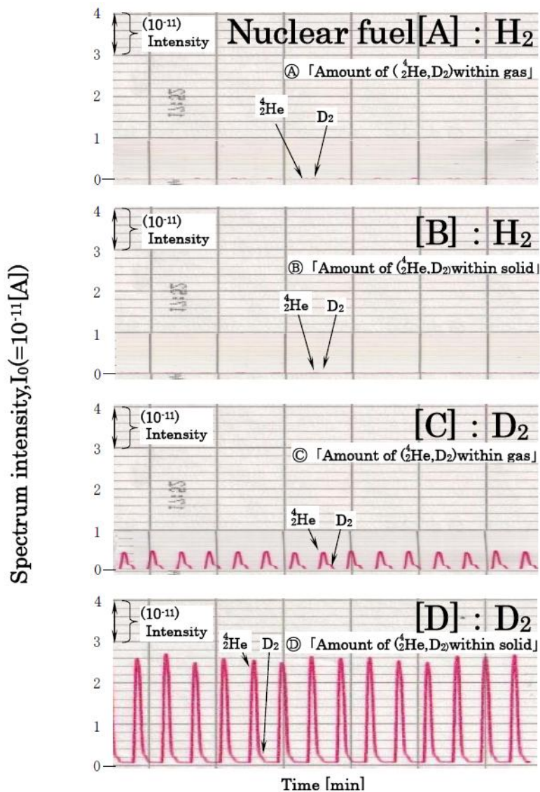
Figure I - 2 QMS mass spectroscopy data: cases [A] and [B] show relative concentration of ^4\text{He} found in the gas and the powder as a result of hydrogen exposure, while [C] and [D] show ^4\text{He} concentration in the gas and the powder due to deuterium exposures (Arata & Zhang, 2008).
