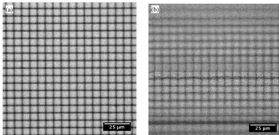
Fig. 8. (a) Image of the grid target acquired using galvo scanners, the grid spacing in the target is 7.5\mu\text{m} . (b) Image of the grid target acquired using EWOD prism raster scanning after distortion correction. The warping in the image is corrected by vector field mapping using a shape preserving spline interpolant function.
