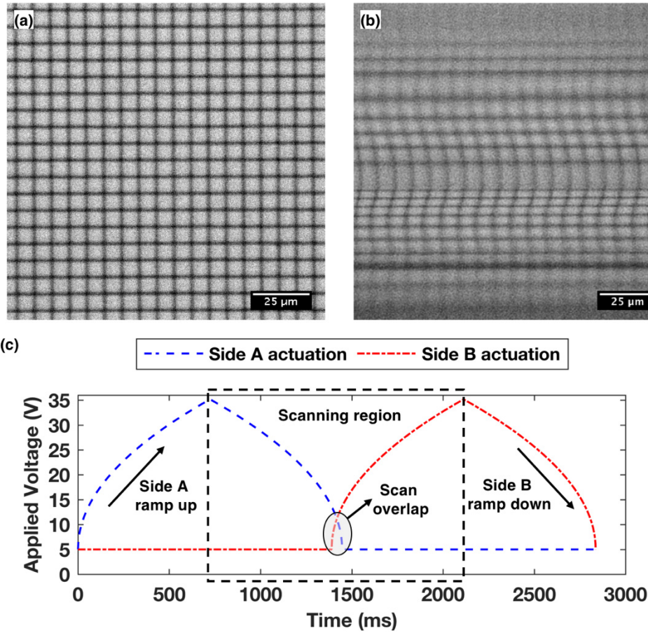
Fig. 7. (a) Image of the grid target acquired using galvo scanners, the grid spacing in the target is 7.5\mu\text{m} . (b) Image of the grid target acquired using EWOD prism raster scanning, the distortions are a result of non-linearity in the scan. (c) Actuation function used to drive the EWOD prism, the function shown in Eq. (2) is alternately applied to both electrodes.
