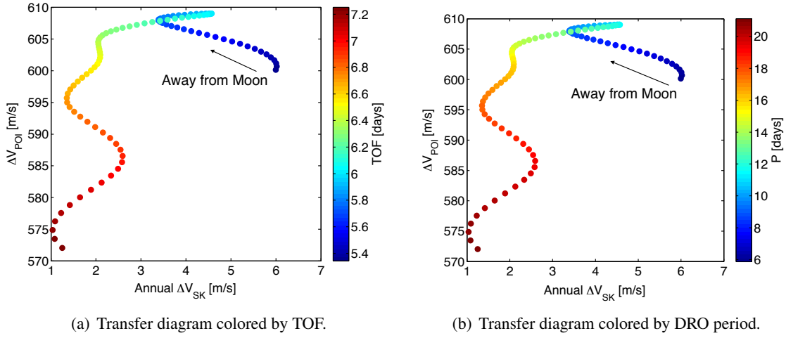
Figure 12. Diagram of transfer and annual station-keeping costs for orbits sampled along the DRO family.
