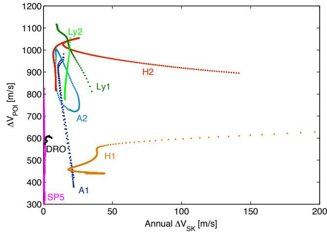
Figure 11. Characteristic curves of transfer and station-keeping cost of each family.
