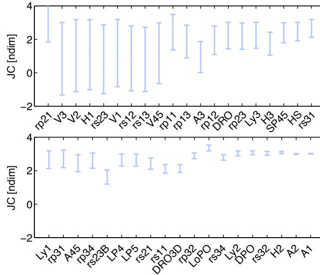
Figure 7. Bar representation of the Jacobi constant of all families available in the reference catalog.
