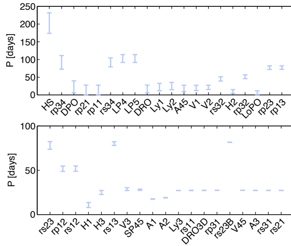
Figure 9. Composite representation of period of the orbits in the families available in the reference catalog.
