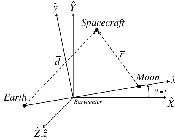
Figure 1. Definition of the rotating coordinate frame with a constant angular velocity relative to the inertial frame at a nondimensional rate of unity about the \hat{Z} -axis.
