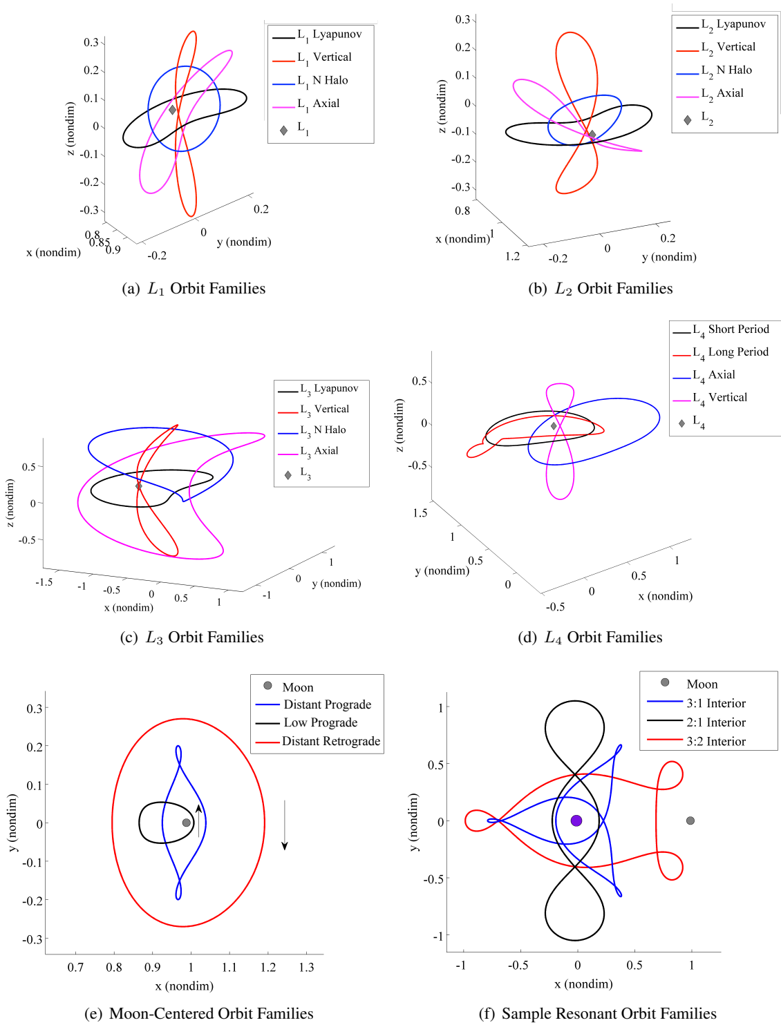
Figure 4. Sample members of well-known orbit families in the Earth-Moon system, plotted in the rotating frame.
