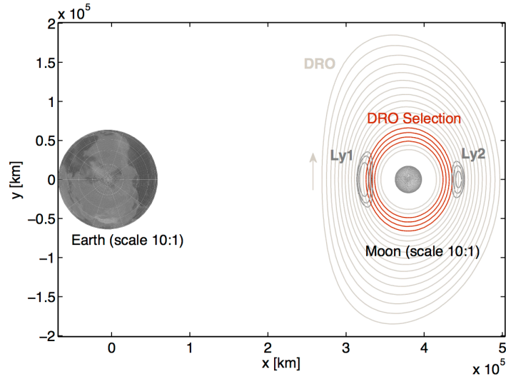
Figure 13. DRO family in the Earth-Moon system with potential storage orbit candidates colored red.
