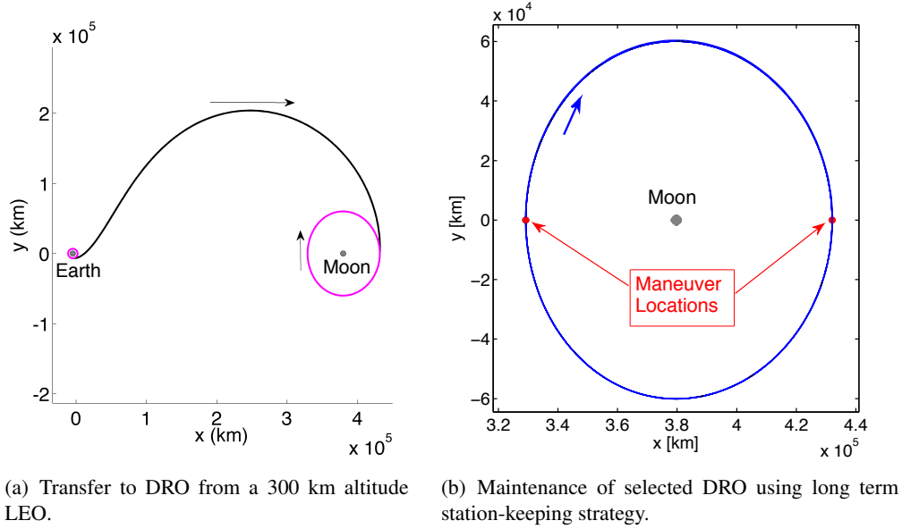
Figure 14. Selected candidate storage orbit, a DRO with period of 9.39 days.
