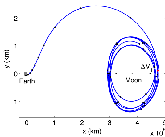
Figure 15. Sample LEO to DRO transfer converged in an ephemeris model for a departure epoch of January 01, 2021 [With permission 21 ].
