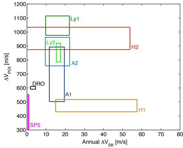
Figure 10. Simplified representation of transfer and station-keeping cost of each family using boxes.
