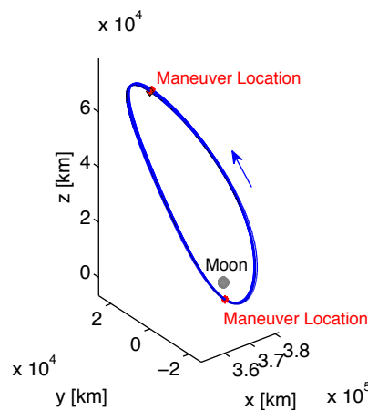
Figure 2. Maintenance of an L_1 halo orbit via long term station-keeping.
