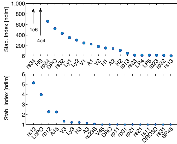
(a) Composite dot representation of the stability index across all families.
