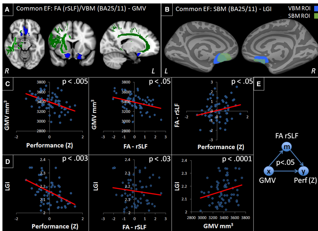
Fig. 1 a Correlations of common EF performance (slice z = -16 , y = 32 , x = 4 , MNI), regional GMV (blue) and FA values (green). b Correlations of common EF performance and regional LGI. Blue VBM – GMV ROI warped onto the FreeSurfer inflated brain, translucent green = SBM – LGI ROI to illustrate the overlap between VBM and SBM findings. c Scatter plots for GMV (mm 3 ) with common EF performance (z score), with FA value, and common
