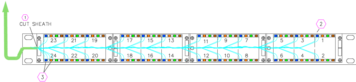
25pr TIE CABLE TERMINATION DETAIL
