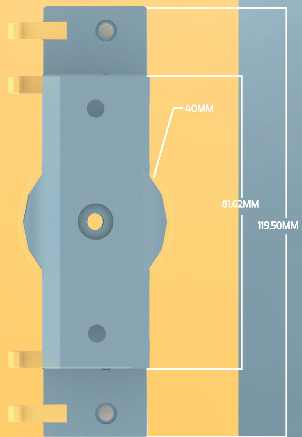
TOP VIEW
