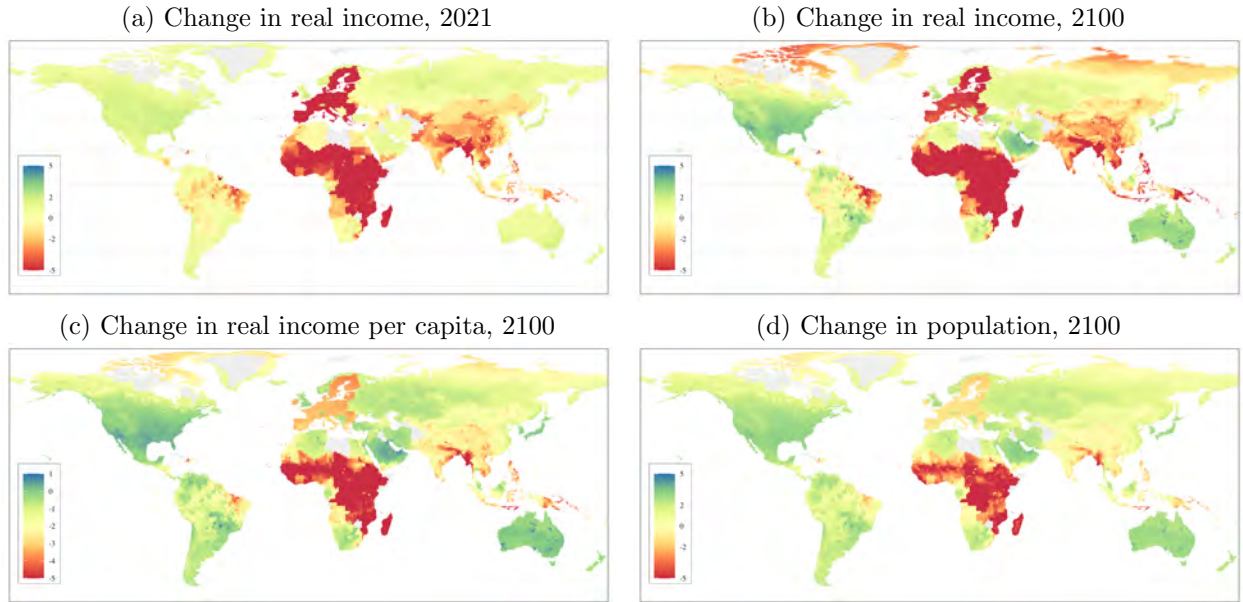
Figure 5: Effect of Carbon Tax and Real Income and Population across the Globe (No Rebating)
