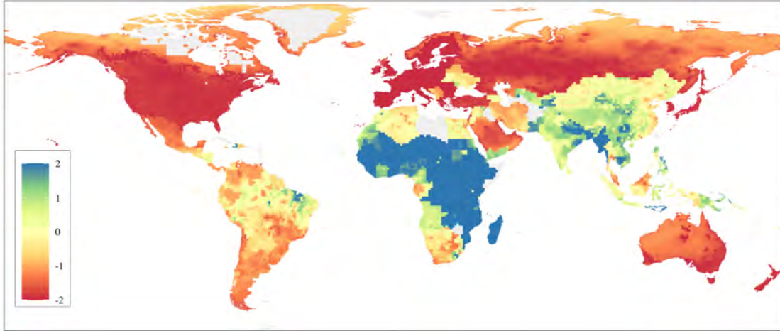
(b) \% \Delta non-agric., dev. countries – local rebating, 2021
