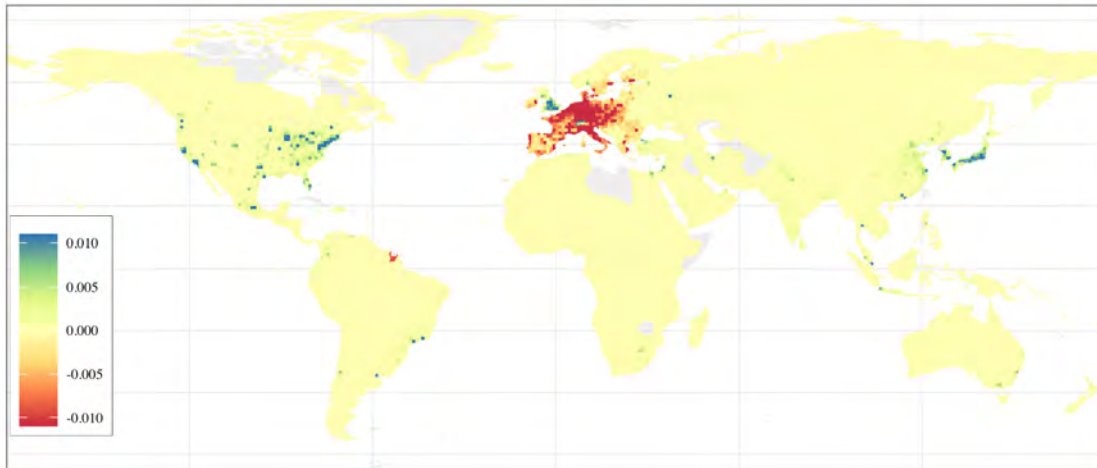
(b) Change in emissions, 2100
