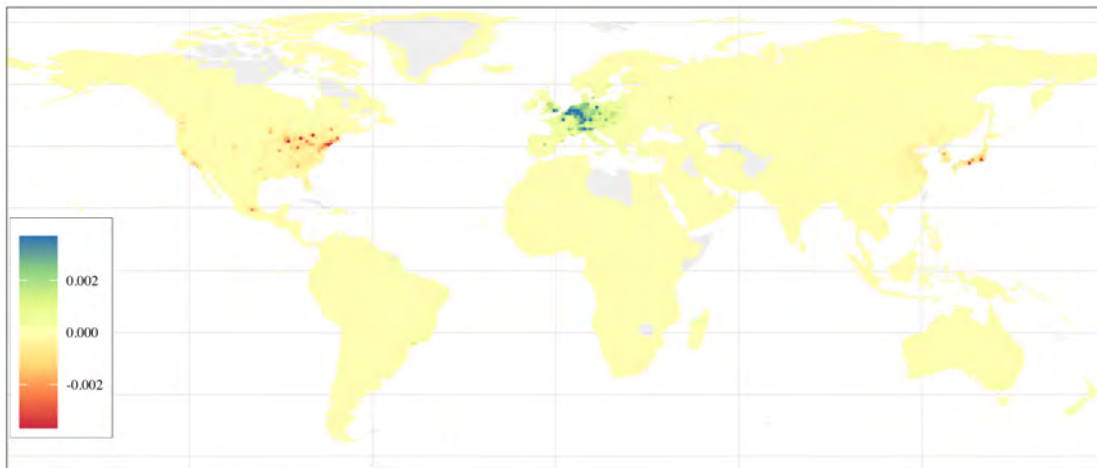
(b) \Delta emissions (local - no rebating), 2100
