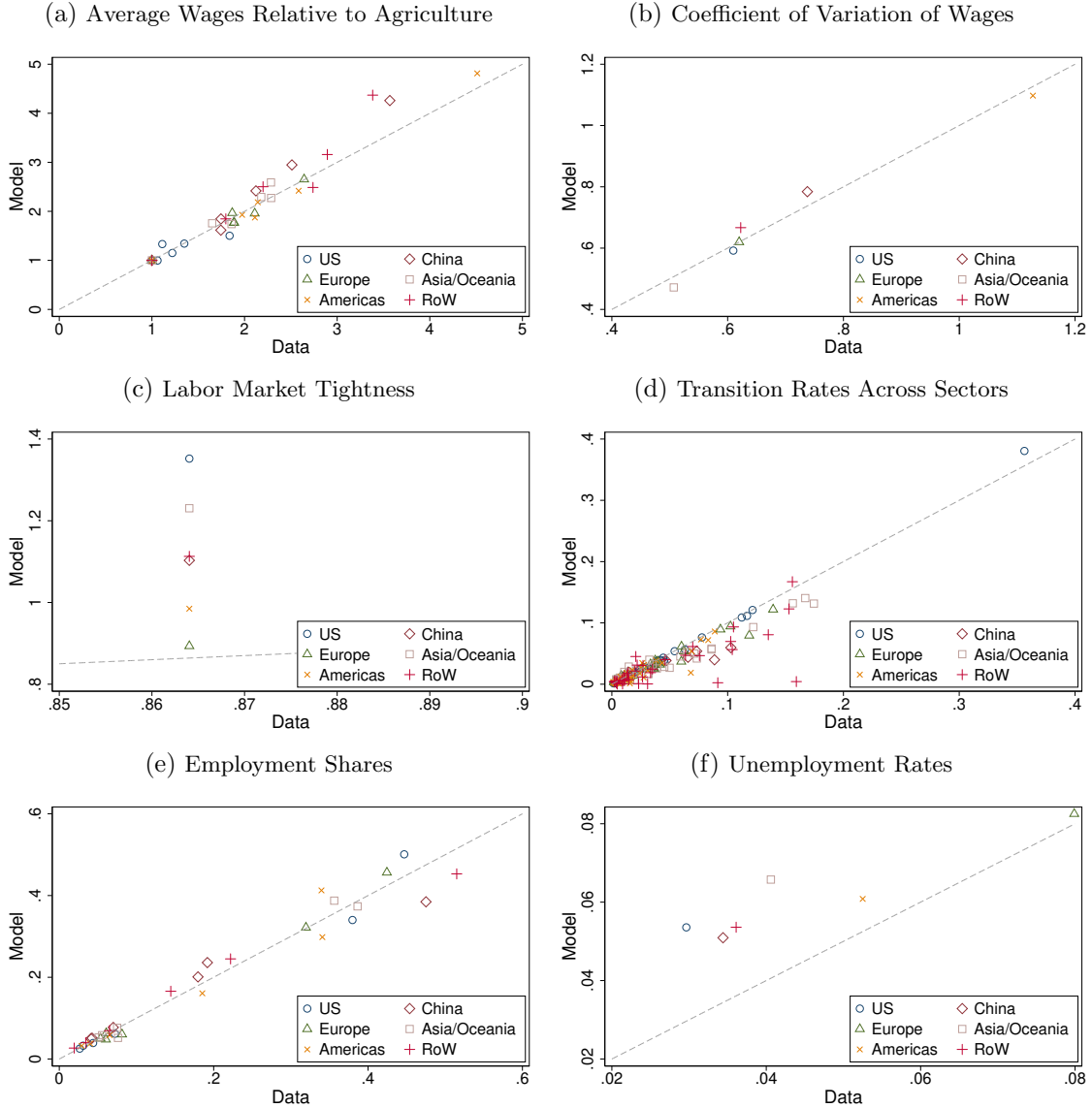
Figure 2: Model Fit
