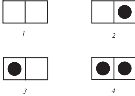
Figure 4. All configurations of a TASEP on a one-dimensional lattice with just two sites. Particles are denoted by black circles.
