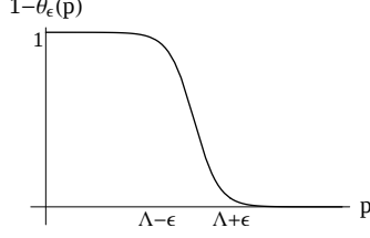
Figure 2.1: A typical cut-off function in the Wilson-Polchinski approach.
