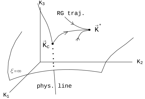
Figure 1.3: Schematic representation of continuous RG trajectories on the critical surface. The flow converges to the fixed point \vec{K}^* . For a given model, the “physical line” corresponds to a change of the temperature. It is not a RG trajectory. For a more precise description of the RG flow, see Fig.2.14.
