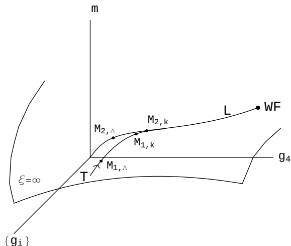
Figure 2.16: Flows on the critical surface for two different initial conditions M_{1,\Lambda} and M_{2,\Lambda} \in L differing only by the initial value of an irrelevant coupling. During the transient regime on T , that is before T is close to L , the RG flows differ between the two trajectories so that at scale k the points M_{1,k} and M_{2,k} are not close to each other although k \ll \Lambda and M_{1,k} is almost on L .
