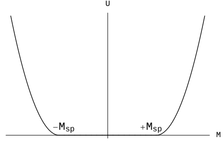
Figure 2.11: Shape of the effective potential U = U_{k=0} for T < T_c .
