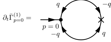
Figure 2.7: Diagrammatic representation of \partial_t \bar{\Gamma}_k^{(1)} evaluated in a uniform field configuration.
