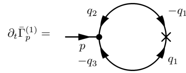
Figure 2.6: Diagrammatic representation of \partial_t \Gamma_k^{(1)} .
