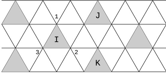
Figure 1.1: Partition of the triangular lattice in plaquettes. The plaquettes are labelled by capital letters I, J, K, \dots and the spins inside the plaquettes are denoted, in obvious notations, S_i^I , i = 1, 2, 3 . The lattice of plaquettes is again triangular with a lattice spacing a\sqrt{3} .
