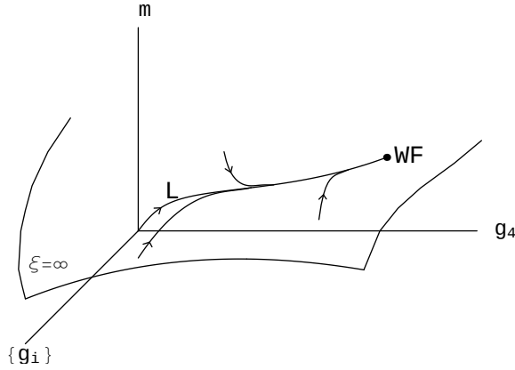
Figure 2.14: Flow on the critical surface. The line L , called the large river, is an attractive submanifold of the RG flow of dimension one (in the Ising case). It starts at the Gaussian fixed point and ends at the Wilson-Fisher fixed point (WF). All RG trajectories approach L very rapidly while the flow on L is “slow”. All the starting points of the RG trajectories correspond to different initial conditions, that is, at microscopic scales, to different \mathbb{Z}_2 -invariant systems. The part of the RG trajectories that is far away from L is non-universal and corresponds to a transient regime. The axis \{g_i\} represents the infinite number of axes different from g_4 which is the coupling of the \phi^4 term. The axis m represents the direction of the mass which is a relevant direction of the RG flow.
