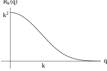
Figure 2.2: A typical cut-off function in the effective average action approach.
