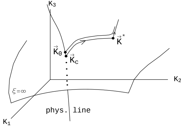
Figure 1.4: Schematic representation of two continuous RG trajectories corresponding to the same model for two different temperatures. The trajectory starting at \vec{K}_c is on the critical surface ( T = T_c ) and the other, starting at \vec{K}_0 , is slightly away from it. There exists a RG trajectory emanating from the fixed point \vec{K}^* and which is not on the critical surface. It is an eigendirection of the RG flow corresponding to the relevant direction. Note that we could parametrize the coupling constant space in such a way that the axis denoted K_3 represents the temperature. It is not necessary that this axis coincides with the relevant eigendirection of the RG flow at \vec{K}^* but it is necessary that it has a non vanishing projection onto this axis since the temperature is for sure a relevant parameter. Note that this is non trivial in an infinite dimensional space.
