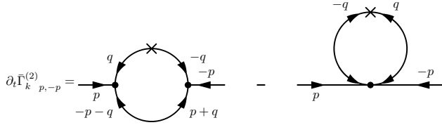
Figure 2.8: Diagrammatic representation of \partial_t \Gamma_k^{(2)} evaluated in a uniform field configuration. Note that the factor \frac{1}{2} has not been represented on the figure for the tadpole because it can be retrieved from the topology of the graph itself (in fact the minus sign can also be retrieved from the graph).
