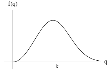
Figure 2.9: The typical shape of the integrand f(q) .
