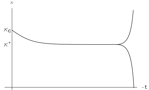
Figure 2.13: Behavior of \kappa(k) very close to \kappa_c .
