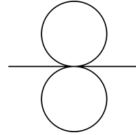
Figure 2.15: The double tadpole diagram contributing to \Gamma^{(2)} and that involves at first order the g_6 coupling. Each tadpole contributes to a factor \Lambda^2 and the vertex (that is g_6 ) to \Lambda^{-2} .
