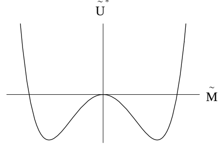
Figure 2.12: Dimensionless fixed point potential of the Ising model in d = 3 . The minima of this potential are located at \pm\sqrt{2\kappa^*} . The spontaneous magnetization is vanishing although \kappa^* \neq 0 (see the text).
