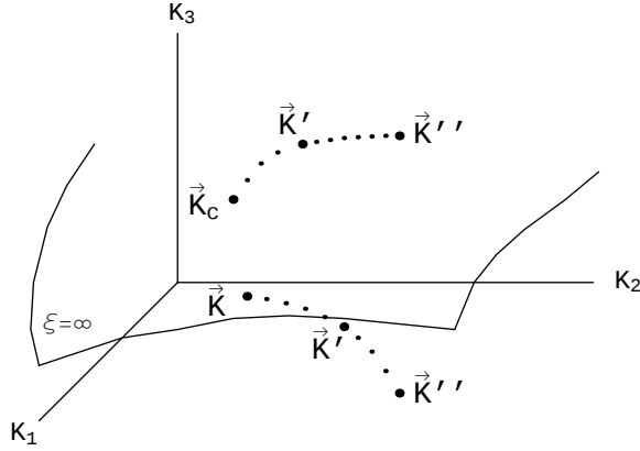
Figure 1.2: Schematic representation of the RG flow in the space of couplings, K_1, K_2, \dots . This space is infinite dimensional and the critical surface, defined by the set of points for which the correlation length is infinite is of co-dimension one. Under RG transformations \vec{K} \rightarrow \vec{K}' \rightarrow \vec{K}'' \rightarrow \dots , the critical surface is stable: if \vec{K} = \vec{K}_c is on the critical surface, then \vec{K}', \vec{K}'' , etc are also on the critical surface. A point away from the critical surface is mapped onto another one “further away” from it.
