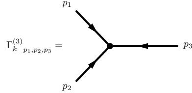
Figure 2.5: Diagrammatic representation of \Gamma_k^{(3)}(p_1,p_2,p_3)[M] .
