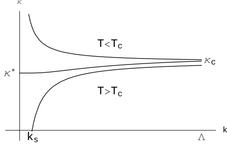
Figure 2.10: Behavior of the running minimum \kappa(k) of the dimensionless potential. From top to bottom: T < T_c , T = T_c and T > T_c . \kappa_c is the critical initial value of \kappa_\Lambda for which the system is critical. This value should not be confused with \kappa^* which is the fixed point value of \kappa(k) . In the low temperature phase the dimensionless running minimum diverges whereas the dimensionful minimum converges to the value of the spontaneous magnetization since it is multiplied by a positive power of the scale k that compensates exactly the divergence of \kappa(k) .
