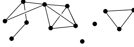
Figure 13.2: A realization of the ER graph of 13 nodes and 14 links. The network is partitioned into four clusters: one of size 8, one of size 3, and two of size 1. There are also one node of degree 5, four of degree 3, four of degree 2, one of degree 1, and two of degree 0.
