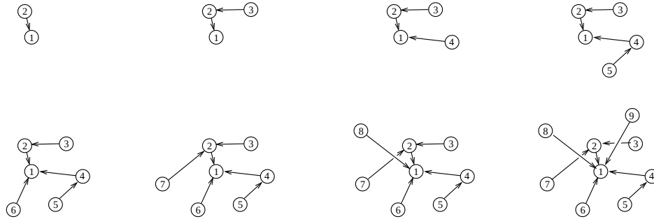
Figure 13.3: Evolution of a representative random recursive tree.
