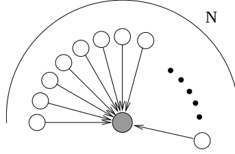
Figure 13.6: Creation of a “bible” in which each new node attaches only to the bible (shaded).
