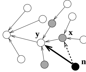
Figure 13.4: Illustration of redirection. The rate at which attachment occurs to the ancestor \mathbf{y} of node \mathbf{x} by redirection is proportional to the number of upstream neighbors to \mathbf{y} (shaded).
