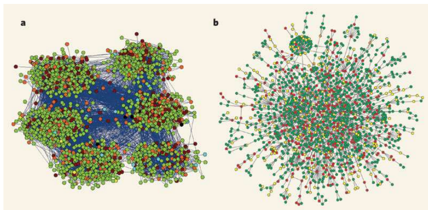
Figure 13.1: Examples of complex networks.
