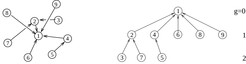
Figure 13.5: A random recursive tree of 9 nodes (from Fig. 13.2) and its corresponding genealogical tree.
