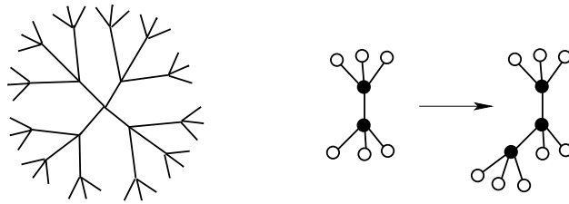
Figure 7.6: (Left) First three generations of a Bethe lattice with coordination number z = 4 . (Right) Counting perimeter sites (circles) starting with a connected cluster of m = 2 and 3 sites (dots).
