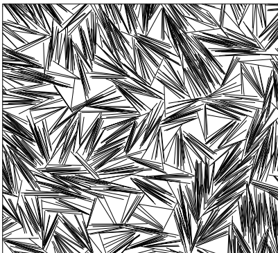
Figure 7.9: Random sequential adsorption of needles in two dimensions.
