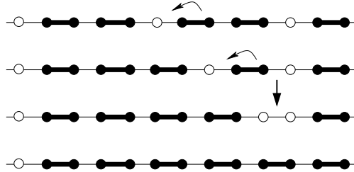
Figure 7.12: Example of mobile adsorbed dimers in one dimension. Each successive row shows the system after a single hopping event. When two holes become adjacent, they are immediately occupied by a dimer.
