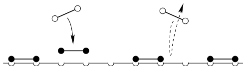
Figure 7.1: Irreversible dimer deposition. The dimer on the left successfully adsorbs onto two adjacent vacant sites, while the dimer on the right does not adsorb.
