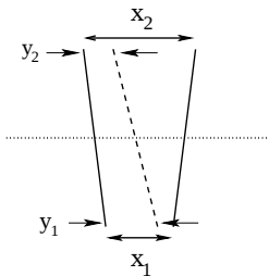
Figure 7.10: Random sequential adsorption of needles in one dimension as the fragmentation of trapezoids.
