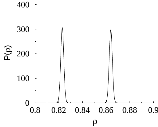
Figure 7.5: The equilibrium distribution (left) and jamming distribution (right) for a system of size L = 10^4 .
