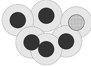
Figure 7.8: Two target areas (white), the exclusion zones (shaded), and the adsorbed disks (dark) near jamming. In the long-time limit only arc-triangular target areas, such as the tiny one on the left, remain.
