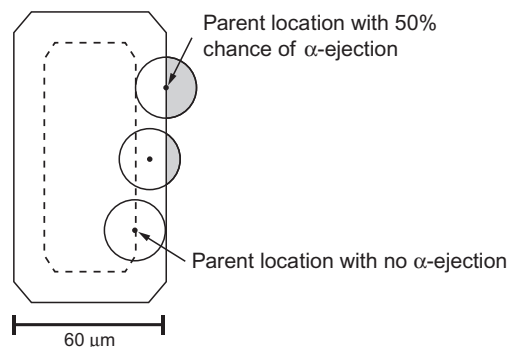
r0010 Fig. 1 Diagram illustrating alpha-ejection in apatite. Each circle represents the \sim 20\ \mu\text{m} distance that {}^4\text{He} atoms travel after being produced during radioactive decay. Shaded portions of the circles represent positions where {}^4\text{He} can come to rest outside the crystal due to ejection, resulting in net {}^4\text{He} loss from the grain. The dashed line shows the volume of the grain where {}^4\text{He} will not be ejected. This volume is a larger proportion of the grain for larger crystal sizes.
