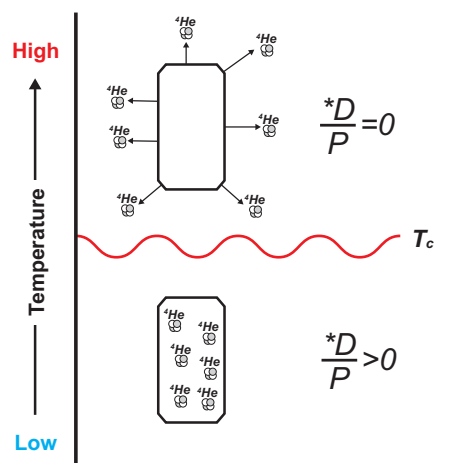
Fig. 2 Schematic diagram illustrating the closure temperature concept. {}^4\text{He} is continuously produced by radioactive decay, but at high temperatures the crystal acts as an open system and {}^4\text{He} will diffuse out of the crystal. Consequently, the radiogenic daughter ( D^* ) to radioactive parent ( P ) ratio is always 0. In contrast, at low temperatures the {}^4\text{He} is retained, and the daughter to parent ratio increases linearly with accumulation time. To first order, for a cooling mineral system, the temperature at which the system transitions from open to closed behavior is referred to as the closure temperature.
