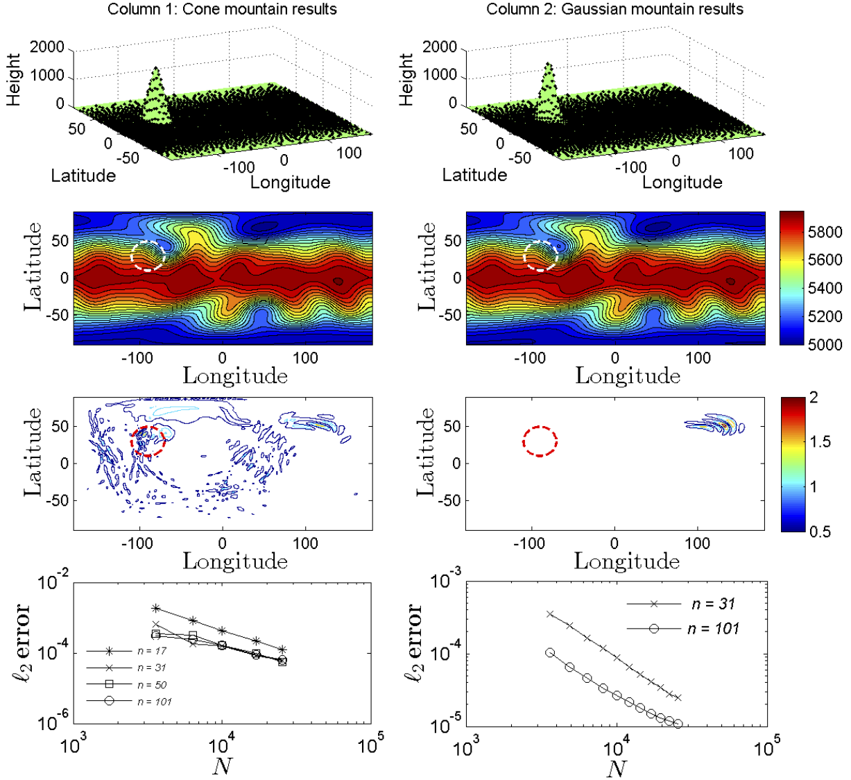
Figure 3: Left column- Cone mountain results: (1) profile of mountain; (2) RBF-FD solution for h at day 15, N = 25,600 and n = 31 with contour intervals at 50 m; (3) magnitude in the error between the RBF-FD solution and DG reference solution; (4) l_2 error as function of the resolution N for varying stencil sizes. Right column, same as left but for the Gaussian mountain forcing. Dashed circle in all plots is the base of the mountain.
