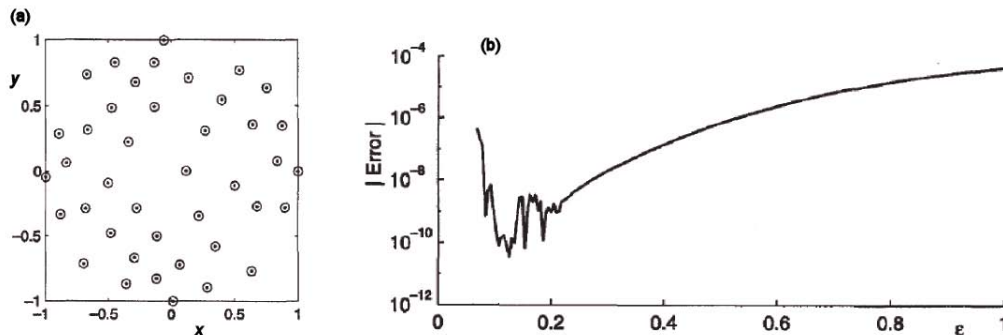
Figure 1: (a) A set of 41 scattered nodes in the unit circle, (b) The error in max norm when the test function f(x, y) = 59/(67 + (x + \frac{1}{7})^2 + (y - \frac{1}{11})^2) is interpolated using these nodes, displayed as a function of the shape parameter \varepsilon . (Reproduced from [17].)
