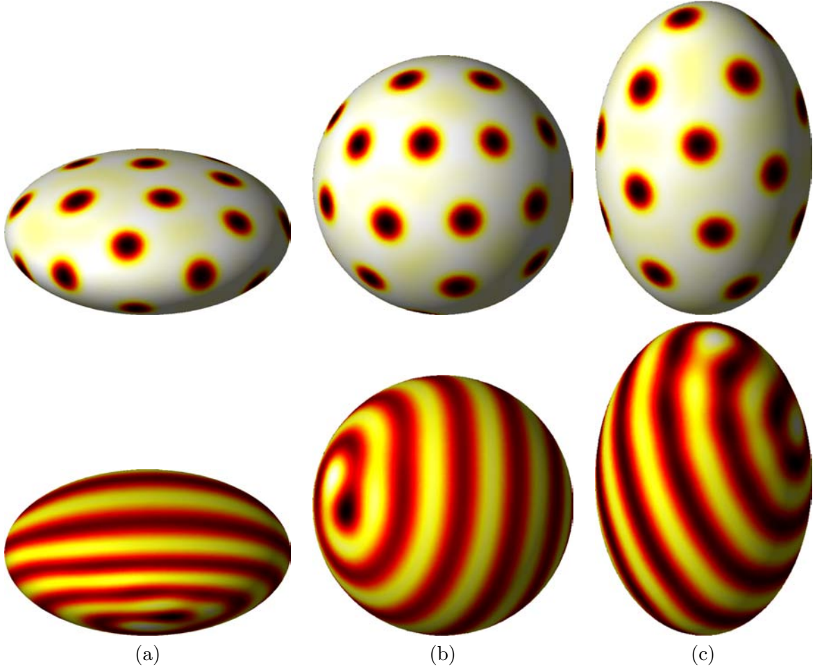
Figure 9: Turing spot and stripe patterns computed from the model (19) on an (a) oblate spheroid, (b) sphere, and (c) prolate spheroid). The pseudocolor plots are for the activator u once steady state is reached. In all plots, black corresponds to a high concentration of u , and white to a low concentration. For all simulations, N = 16,384 and n = 31 , with a time-step of \Delta t = 0.05 . All simulations were run until a steady-state solution was reached, which was about 800 time-steps for the spot patterns and 6000 for the strip patterns.
