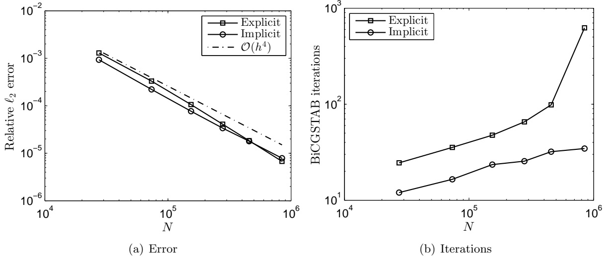
Figure 12: The error and the number of iterations as a function of N .
