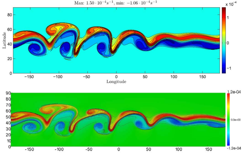
Figure 7: Top: RBF-FD solution for N = 163,842 and n = 31 , Bottom: DG solution at 39 km resolution.
