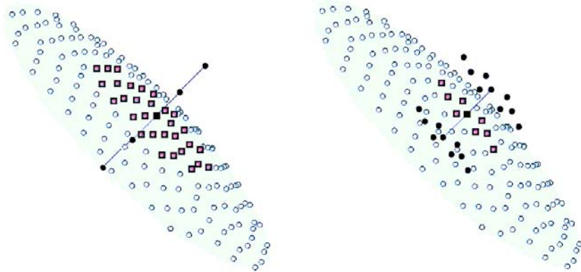
Figure 10: Schematic picture of the two types of stencils. Left panel: Explicit stencil. Right panel: Implicit stencil.
