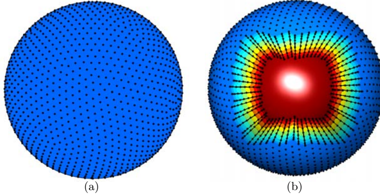
Figure 13: (a) Node layout for the RBF-FD approximations on the surface of a sphere; (b) 3-D view of the discretization of the spherical shell used in the hybrid RBF-FD/Chebyshev calculation. Blue is the outer boundary and red is the inner boundary, black circles display the computational nodes, which are distributed in the radial direction along the extrema of the Chebyshev polynomials. The spherical shell has been opened up in (b) to show the detail of the radial discretization.
