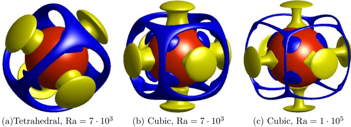
Figure 14: Steady-state isosurfaces of the residual temperature, \delta T , for the three isoviscous benchmark test cases using the RBF-FD model. Here the residual temperature \delta T = T(r, \theta, \lambda) - \langle T(r) \rangle is visualized, where \langle \rangle denotes averaging over a spherical surface. Yellow corresponds to \delta T = 0.15 and denotes upwelling relative to the average temperature at each radial level, while blue corresponds to \delta T = -0.15 and denotes downwelling. The red solid sphere shows the inner boundary of the 3-D shell corresponding to the core.
