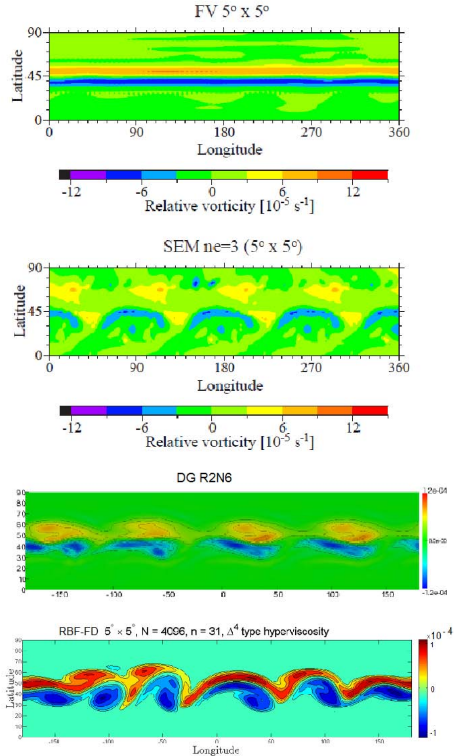
Figure 8: The relative vorticity at day 6 for the evolution of the highly unstable wave case with resolution of 5^\circ \times 5^\circ for a spectral element model (SEM), finite volume model (FV) [49], and the RBF-FD model. The DG model is approximately a resolution of 3^\circ \times 3^\circ . R2 corresponds to 16 elements per face of the cubed sphere for a total of 96 elements, while N6 corresponds using 6 \times 6 = 36 Legendre quadrature nodes. In the SEM model, ne = 3 , corresponds to 3 \times 3 = 9 elements per face of the cubed sphere. In each element 8 \times 8 Gauss-Legendre-Lobatto nodes are used.
