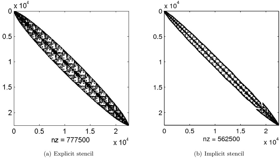
Figure 11: The sparsity pattern for N_H = 2500 , N_R = 11 .
