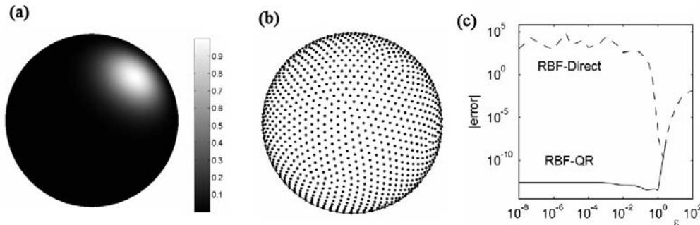
Figure 2: (a) Test function f(x) = e^{-7(x+\frac{1}{2})^2 - 8(y+\frac{1}{2})^2 - 9(z-\frac{1}{\sqrt{2}})^2} , (b) n = 1849 ME (minimal energy) nodes, (c) Interpolation errors (in max norm) when using RBF-Direct vs. using the stable RBF-QR algorithm.
