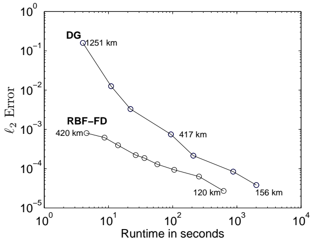
Figure 5: The error as a function of runtime (defined by wall clock time) for the flow over the cone mountain test case.
