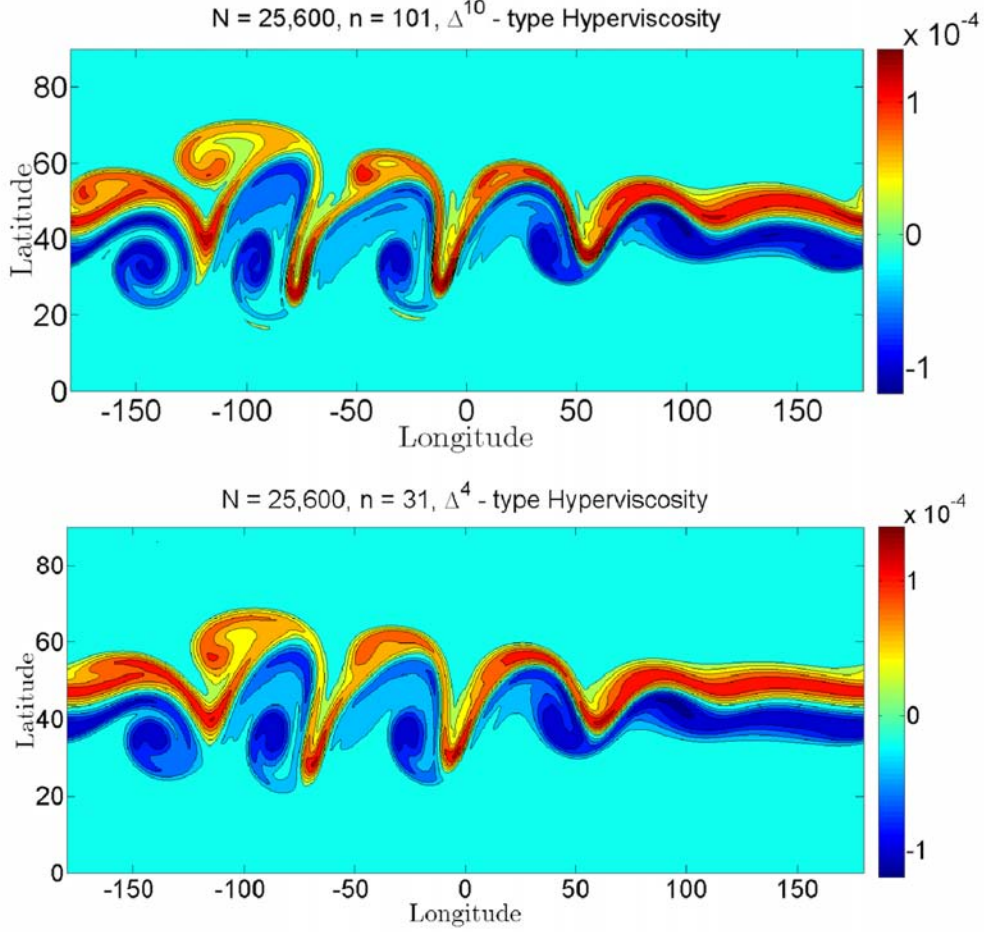
Figure 6: The relative vorticity at day 6 for the evolution of the highly unstable wave case as function of resolution N and stencil size n . Contour interval is 2 \cdot 10^{-5} s^{-1} .
