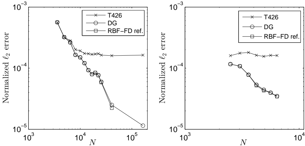
Figure 4: The normalized \ell_2 error in the height field h as a function of N for flow over a conical mountain at day 15 for RBF-FD (left panel) and global RBFs (right panel). The different markers correspond to different reference solutions.
