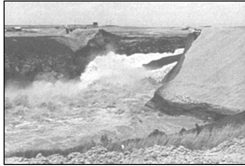
Teton Dam, Idaho failing by internal erosion on June 5, 1976. Left, initial breakout of seepage on face of dam. Middle, wave pouring through eroded opening. Right, after wave passed through.
