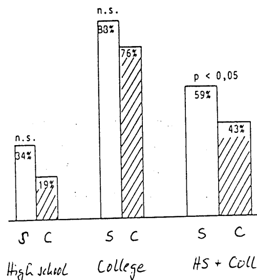
Figure 7: Effects of problem formulation on solution frequencies in the cyclist task.
