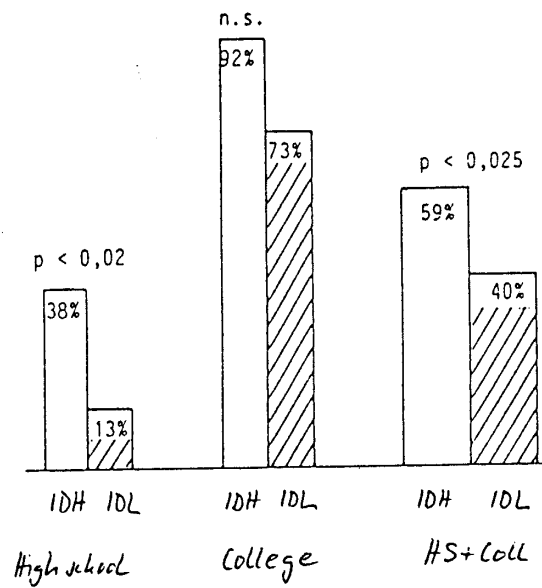
Figure 6: Effects of difficulty induction on solution frequencies in the cyclist task
