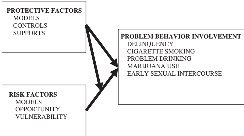
FIGURE 1 Explanatory model of direct effects of protective factors and risk factors on adolescent problem behavior, and moderation of Risk \times Protection.
