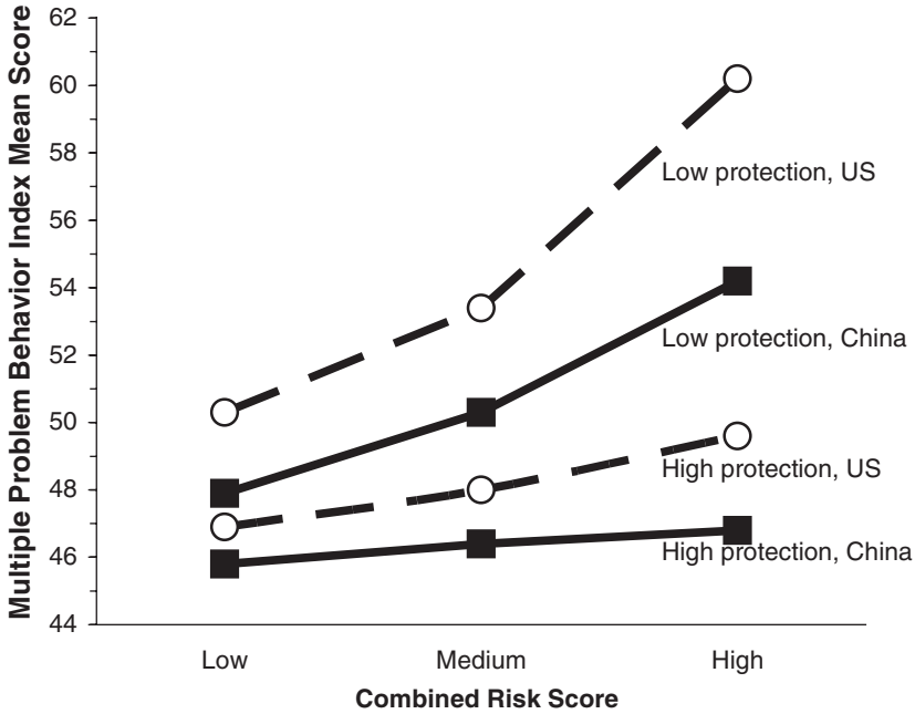
FIGURE 2 Moderation of combined Risk Score \times Controls Protection: U.S. sample and Chinese sample.
