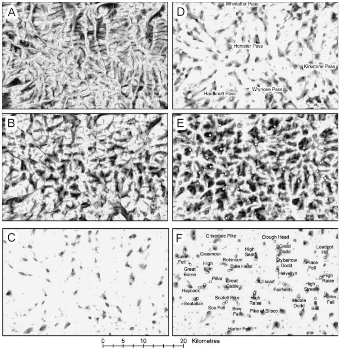
Figure 5 Fuzzy memberships of the six morphometric landforms: (A) planarity; (B) channelness; (C) pitiness; (D) passness; (E) ridgeness; (F) peakness. The locations of toponyms for passes and summits are shown on (D) and (F) (Copyright © Bartholomew, 2002). The feature extractions shown in this figure used a threshold of 4^\circ for the peaks
