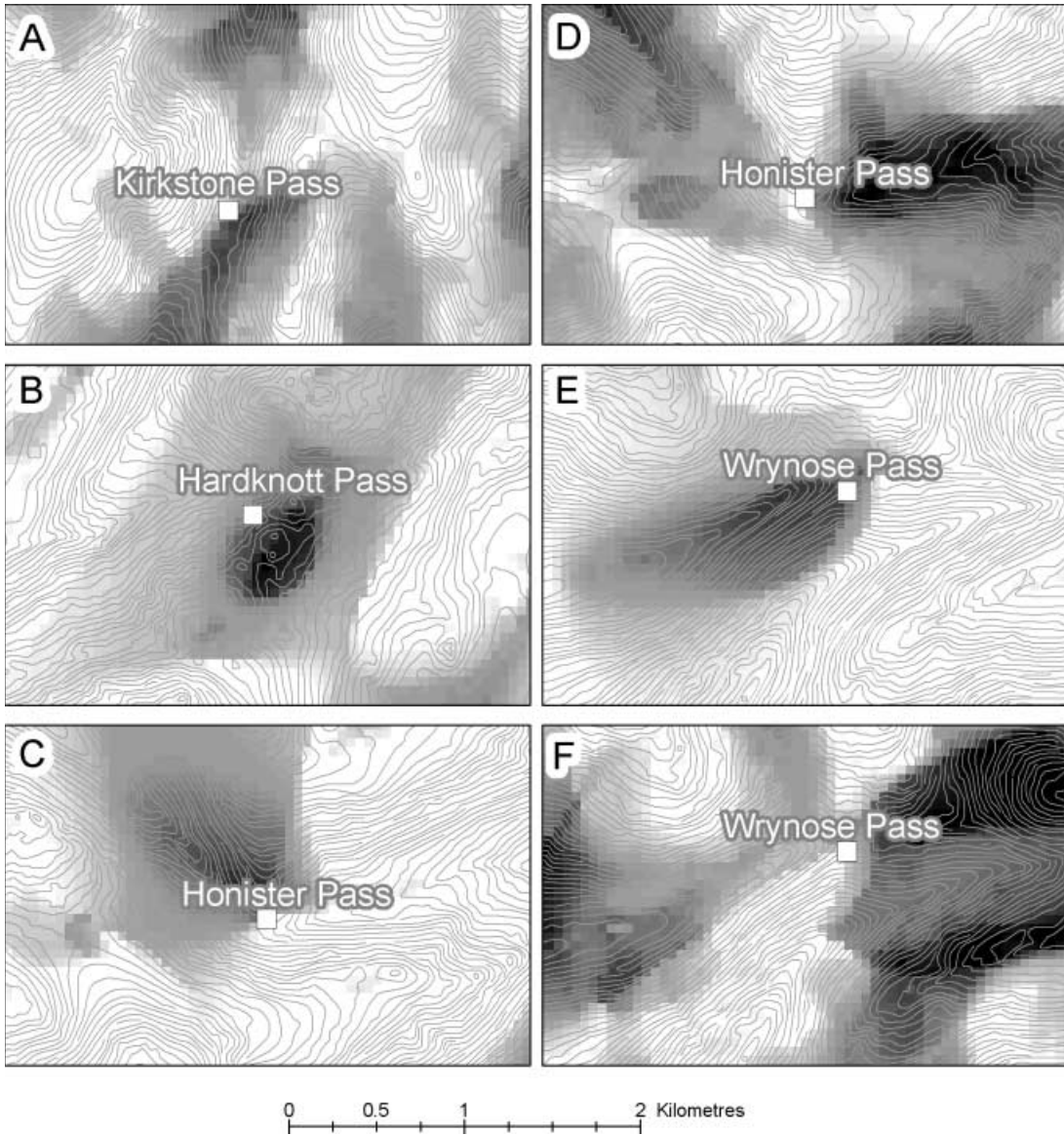
Figure 9 Detail maps of passness in the vicinity of (A) Kirkstone Pass, (B) Hardknott Pass, (C) Honister Pass and (E) Wrynose Pass. The degree of channelness is shown in the vicinity of (D) Honister Pass and (F) Wrynose Pass.
