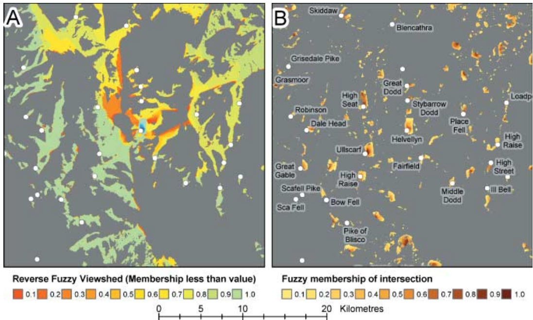
Figure 12 (A) The areas which can see Helvellyn and the degree to which it is possible to see Helvellyn from them (the reverse fuzzy viewshed) based on the 4^\circ threshold for extraction, and (B) the intersection of the reverse fuzzy viewshed of Helvellyn with the degree of peakness, showing the distributions of areas where peaks occur from which it is possible to see Helvellyn
