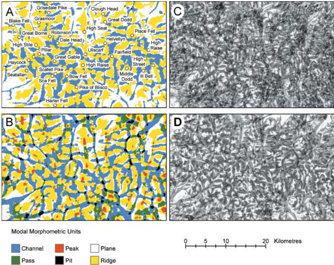
Figure 6 (A) and (B) show modal classes and (C) and (D) the corresponding entropy values when thresholds of 1^\circ and 4^\circ respectively were used in extraction of morphometric features
