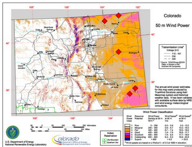
Figure 2: Location of wind sites for five-site model (locations marked with diamonds) [9]
