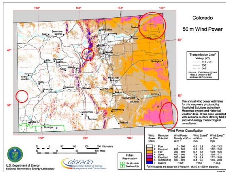
Figure 1: CAES site possibilities in Colorado [9]
