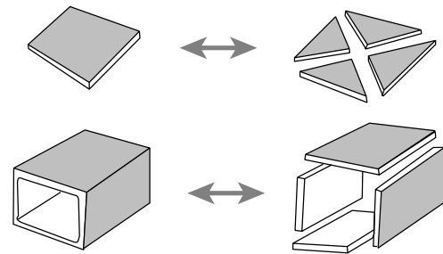
FIGURE 6.7. Macroelement examples.
