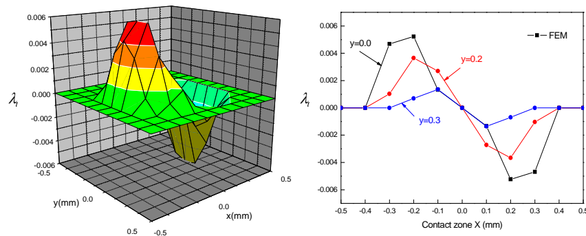
Figure 6. Distribution of tangential multipliers with \mu = 0.25 and the normal load N applied with ten time steps.
