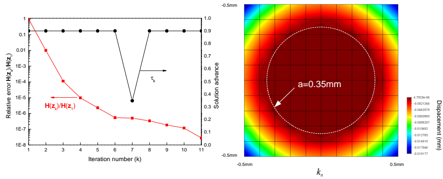
Figure 4. Convergence rate of the GNMLS algorithm and normal distance k_n between the deformed spheres and the frame.
