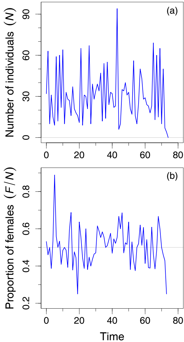
Figure 3. One Monte Carlo simulation of a stochastic Ricker model with several sources of demographic variance, including stochastic sex determination. The population went extinct after 74 generations. (a) Fluctuations in total population size. (b) Fluctuations in the proportion of females. The model is the WSB model in Fig. 2 with the same details.
