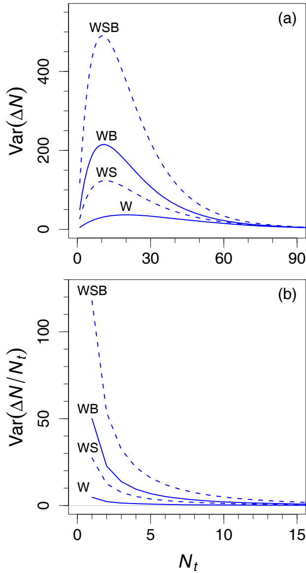
Figure 2. How sources of demographic variance combine together to cause variance in population size illustrated with a stochastic Ricker model. In this example, sources of demographic variance can be divided into contributions from probabilistic births and deaths at the within-individual scale (W), probabilistic sex determination (S), and differences in female fecundity at the between-individual scale (B). (a) Stochastic
