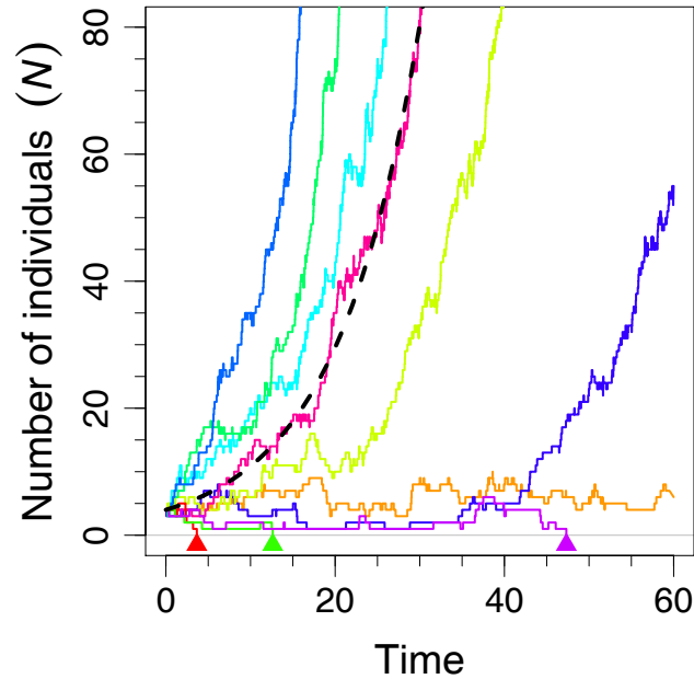
Figure 1. Demographic stochasticity caused by probabilistic births and deaths of discrete individuals. Variation from demographic stochasticity is illustrated here by ten representative realizations of population growth from 1000 Monte Carlo simulations of the same stochastic model. Dynamical outcomes included populations that experienced exponential growth (some fast, some slow), populations that experienced a long period of low population size before exponential growth occurred, populations that did not grow at all during the period, and 62 populations that went extinct. This contrasts with the equivalent deterministic model of exponential growth (dashed black line). Of simulations that did not go extinct, shown are the simulations with the highest and lowest number of individuals at the end of the simulation, as well as the 2.5th, 25th, 50th, 75th, and 97.5th percentiles. Of simulations that went extinct, shown are the shortest, median, and longest extinction times. Triangles show the time of extinction. Model details: individuals were identical and reproduced asexually; births and deaths were density independent with rates
