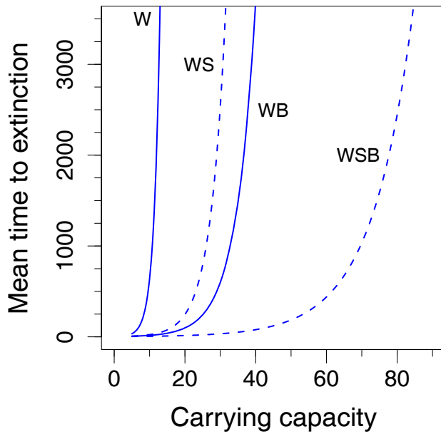
Figure 4. The mean time to extinction increases exponentially with carrying capacity due to demographic stochasticity. Populations go extinct more rapidly when the carrying capacity is low. The example is a stochastic Ricker model as in Fig. 2. Compared to probabilistic births and deaths alone (W), extinction risk is increased by probabilistic sex determination (WS) and when fecundity differs between females (WB, WSB). Model details were the same as in Fig. 2 except: variation in intrinsic birth rate between females was gamma with mean 10 and variance 10; density independent mortality was Bernoulli with probability 0.6.
