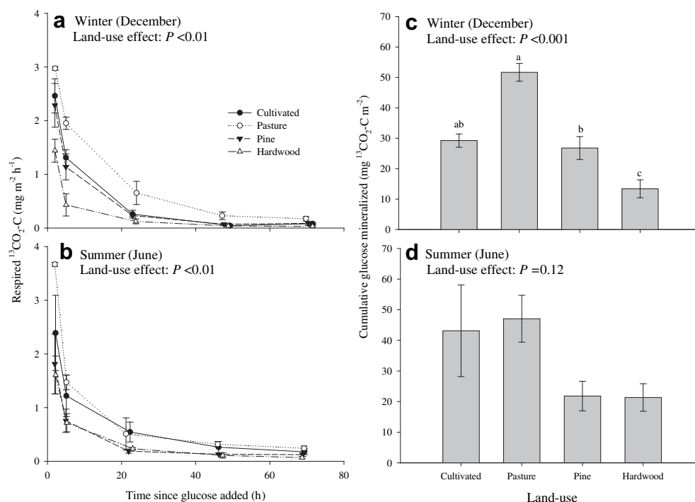
Fig. 1. Results of the 13 C-glucose pulse-chase conducted during the winter (December 2006) and summer (June 2007) associated with land-use. Panels a and b show glucose mineralization dynamics across 72 h for each land-use. Land-use differences were detected for these dynamics across seasons ( P < 0.01 ) and during both the winter ( P < 0.01 ) and summer ( P < 0.01 ). Panels c and d show the cumulative amount of glucose mineralized during the entire 72-h period. Although there was a significant land-use effect across seasons on cumulative glucose mineralization ( P < 0.01 ) this was not consistent within seasons. That is, a statistically significant land-use effect was observed in the winter ( P < 0.001 ) but not in the summer ( P = 0.12 ) for cumulative amounts. Values are means \pm S.E. per land-use ( n = 3 ) and letters in panel c indicate significant differences between land-uses based on pair-wise comparisons. Note that mineralization dynamics and cumulative values were roughly equivalent for a given land-use regardless of season.
