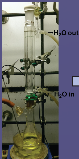
Water condenser
