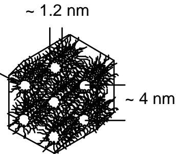
nanostructured polymer network
