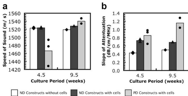
Fig. 7. SoS and SoA as a function of in vitro culture period for (white bars and diamonds) ND hydrogels without cells, (dark gray bars and triangles) ND constructs with encapsulated chondrocytes and (light gray bars and circles) PD constructs with encapsulated chondrocytes, calculated from 100 MHz transducer data. Averages are shown by bars and individual measurements are also shown for each time point and condition.
