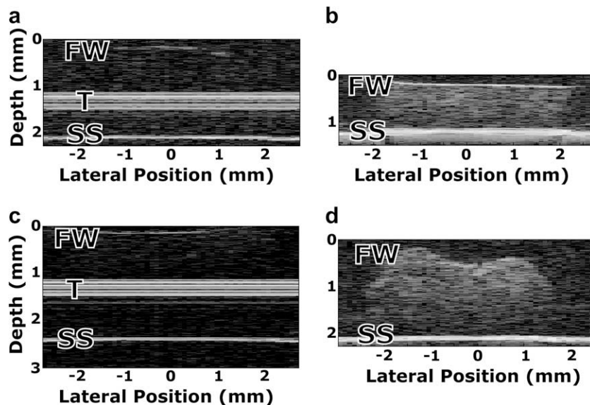
Fig. 6. B-Scans of (a) hydrogel only, (b) bovine cartilage explant, (c) PD cell-gel construct after three days of in vitro culture and (d) PD cell-gel construct after 9.5 weeks of in vitro culture. Labels correspond to the front wall (FW) of the sample being tested, the transducer delay rod artifact (T) and the stainless steel plate (SS) on which the samples rested during testing. Data for the images in panels (a and c) were collected with a 100 MHz transducer, while data for the images in panels (b and d) were collected with a 50 MHz transducer.
