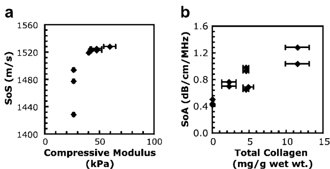
Fig. 8. Scatter plots of (a) SoS plotted against compressive modulus measurements and (b) SoA plotted against total collagen density. SoS and SoA were calculated from 100 MHz transducer data.
