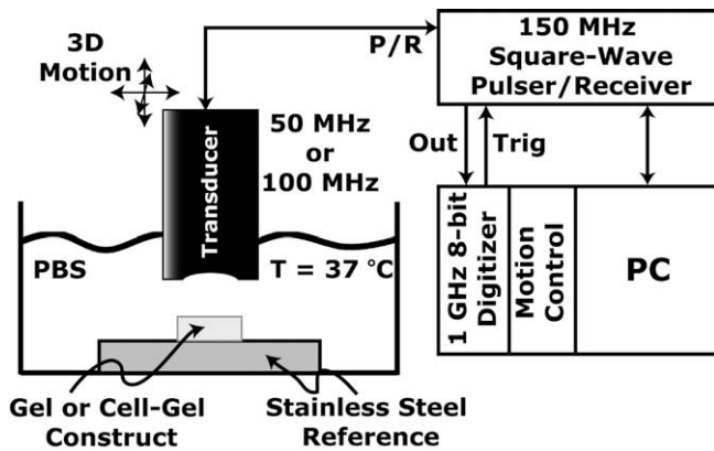
Fig. 1. High-frequency ultrasound setup. Measurements of tissue specimens were performed with either a 50 or a 100 MHz transducer that was electrically excited by a 150 MHz square wave pulser/receiver (P/R). Received signals were digitized at a rate of 1 GSamples s^{-1} with 8-bit resolution. Motion control and data acquisition were automated by PC control. Tissue specimens were immersed in a phosphate-buffered saline (PBS) solution that was heated to 37 °C and mounted on a custom, stainless steel fixture.
