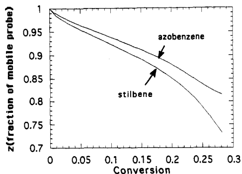
Figure 3. Fraction of probes that are mobile as a function of double-bond conversion of TrMPTrMA polymerized with 1.2 mW/cm 2 of UV light and 1 wt % DMPA.
