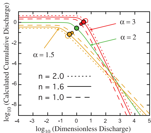
Figure 7. Effect of errors in n , defined by (3) and used in (10), on theoretical values of \log_{10} [365D'(Q' \geq Q^*)] versus \log_{10} Q^* , for three values of \alpha . As shown in (10), if \alpha = 2 , D'(Q' \geq Q^*) is independent of n . Larger values of n enhance climatic differences, manifested by different \alpha .
